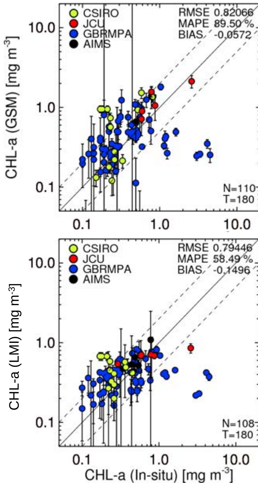
Figure 87: MODIS Aqua Chlorophyll-a retrieval vs. in situ data. Only the measurements collected within \pm 3 hours time difference to the overpass were plotted. Number of matchups are 108 for LMI and 110 for gsm.
