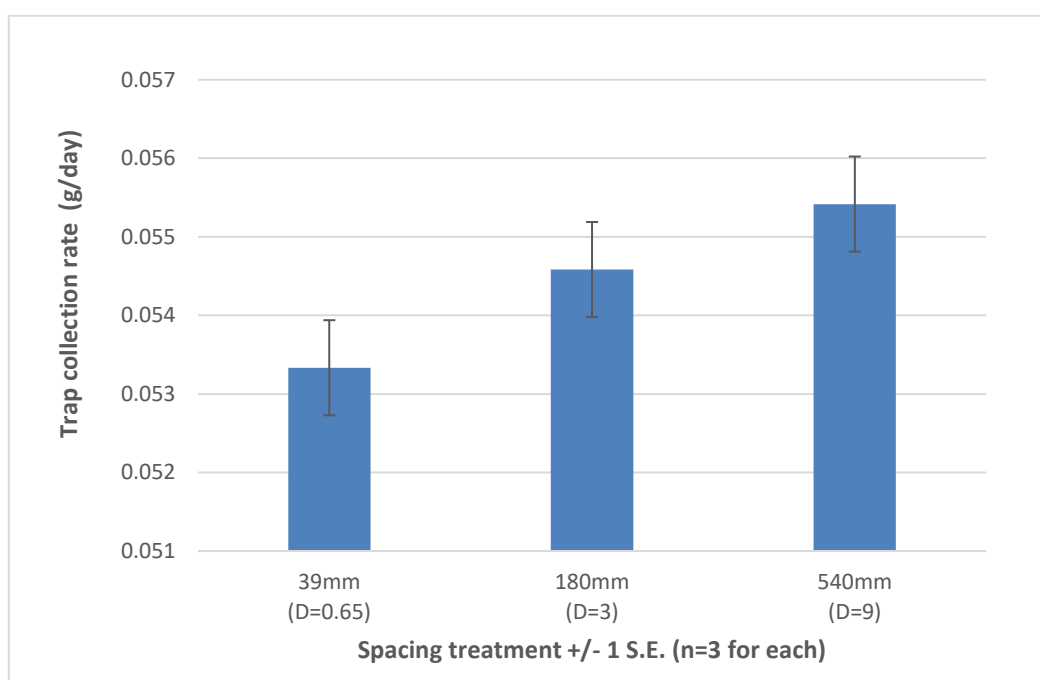
Figure 2.21. Sediment trap collection rates from a circular flume experiment with trap spacing of 0.65D, 3D and 9D.
