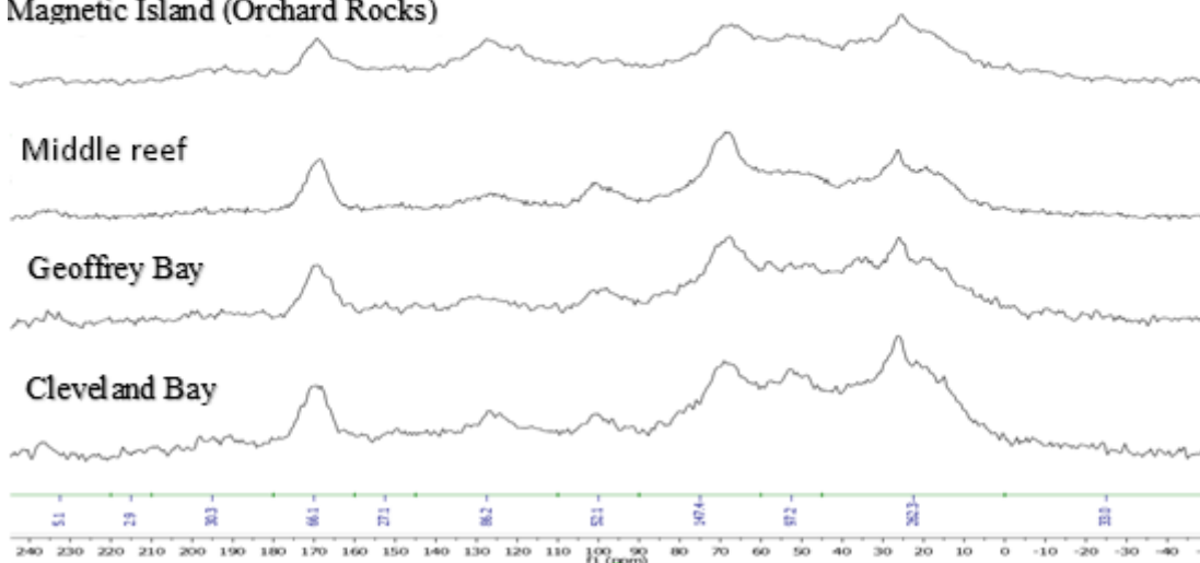
Figure 5.4B. Chemical composition of organic matter in marine sediments collected from different sediment traps (Magnetic Island, Middle reef, Geoffrey Bay, Cleveland Bay) as revealed by ^{13}\text{C} NMR CP MASS.
