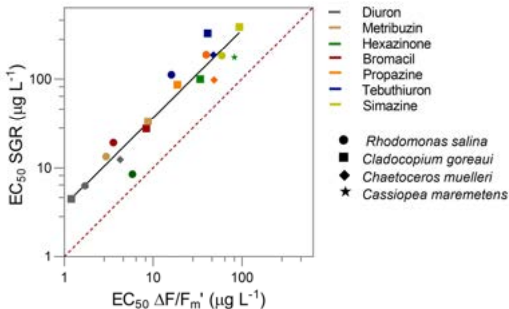
Figure 1. Linear relationship between inhibition of growth and inhibition of effective quantum yield ( \Delta F/F_m' ) for marine taxa. Comparison of EC_{50} values [ EC_{50}(SGR) = 3.36 * EC_{50}(\Delta F/F_m') + 13.2 ; R^2 = 0.72 ] of seven PSII herbicides to four species. Dashed line indicates 1:1 relationship.
