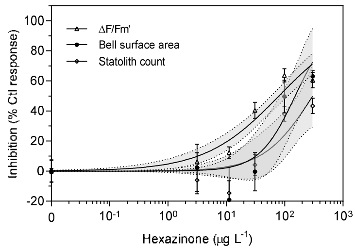
Figure A1. Sigmoidal, 4-parameter curve fit and 95% confidence intervals (shaded area) on the relative percent inhibition of 14-day effective quantum yield ( \Delta F/F_m' ), bell surface area, and statolith count of C. maremetens (mean \pm SEM) following herbicide exposure to hexazinone at increasing concentrations. All concentrations are reported in \mu\text{g L}^{-1} ( n = 15 for each treatment for \Delta F/F_m' , and n = 5 for each treatment for both bell surface area and statolith count, bars not visible are smaller than symbol).
