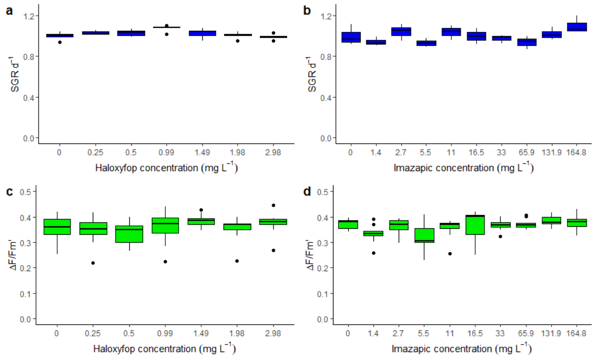
Figure A3. Boxplots of the specific growth rate (SGR d -1 ) and effective quantum yields (ΔF/Fm') of Cladocypium goreau in response to haloxyfop (a, c) and imazapic (b, d). All concentrations in mg L -1 .
