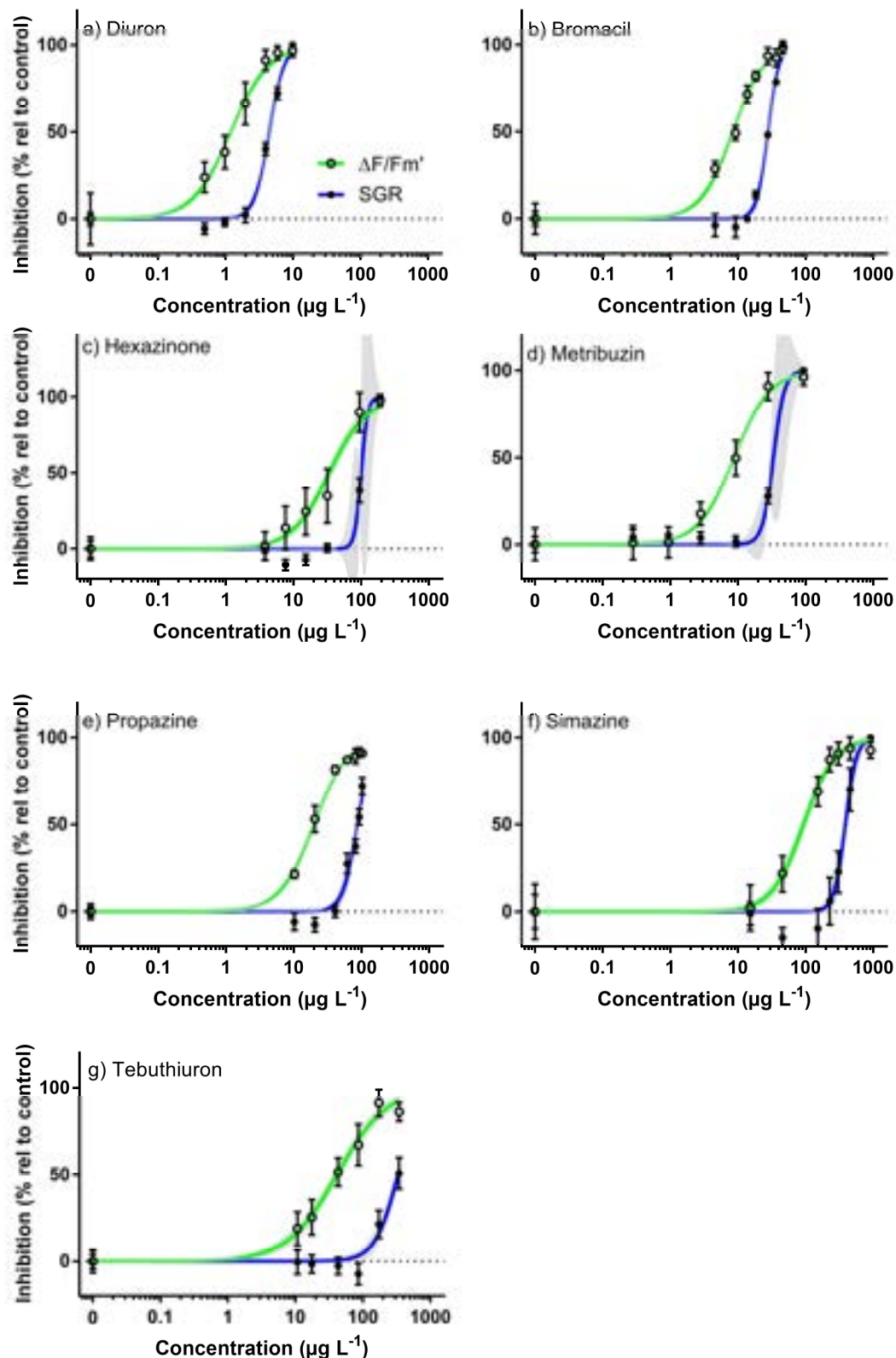
Figure A1. Concentration-response curves for \text{EC}_x derivation. Sigmoidal, 4-parameter curve fit (solid line) and 95% confidence intervals (shaded area) on the relative percent inhibition of 14-day specific growth rate (SGR; closed circle, mean \pm SD) and effective quantum yield ( \Delta F/F_m' ; open circle, mean \pm SD) of Cladocopium goreau following herbicide exposure to a) diuron; b) bromacil; c) hexazinone; d) metribuzin; e) propazine; f) simazine; and g) tebuthiuron at increasing concentrations. All concentrations in \mu\text{g L}^{-1} (error bars not visible are smaller than symbol).
