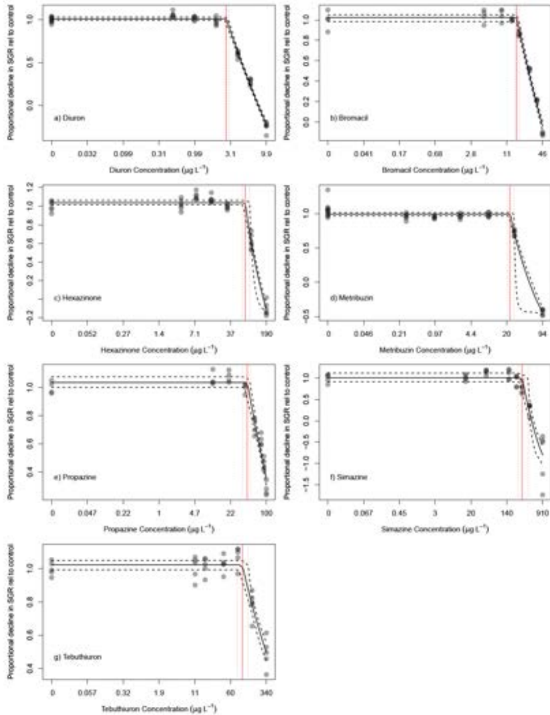
Figure A2. Bayesian non-linear gaussian model fits (except for propazine in which a gamma model was a better fit) on the proportional decline of specific growth rate (SGR) of Cladocopium goreaui relative to the control treatment (solid black line) and 95 % confidence intervals (black dashed line) and the derived no effect concentration (NEC) (red line) and 95% confidence interval (red dashed line) of a) diuron; b) bromacil; c) hexazinone; d) metribuzin; e) propazine; f) simazine; and g) tebuthiuron. All concentrations in \mu\text{g L}^{-1} .
