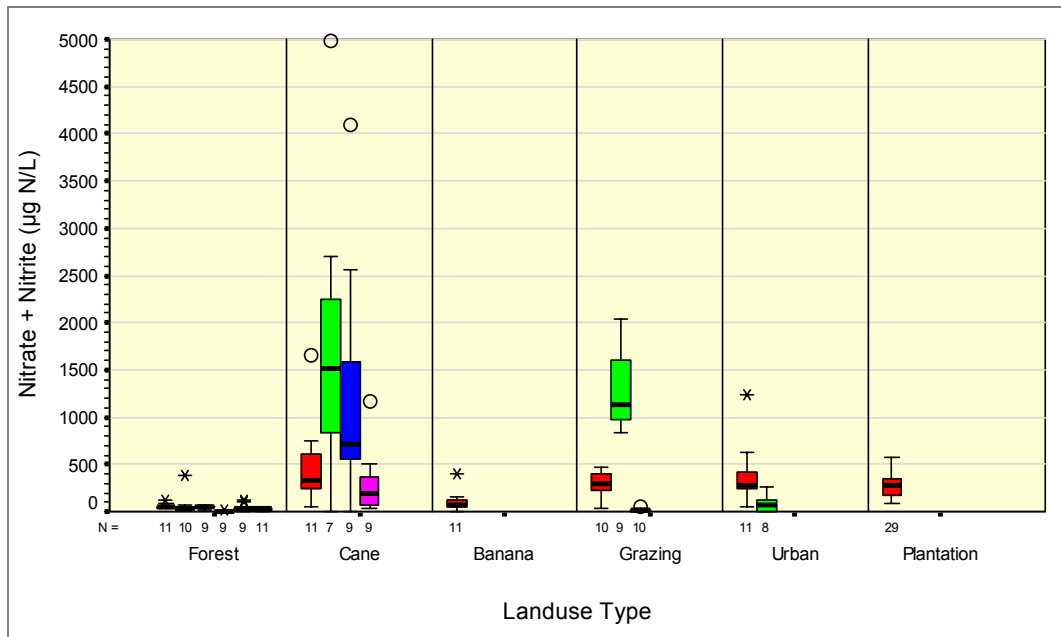
Figure 5: A boxplot showing the relative distribution of nitrate + nitrite ( \text{NO}_x ) ( \mu\text{g N/L} ) in river and creek flows for the five land use activities within the Tully-Murray Rivers region between December 2005 and July 2006. Plantation \text{NO}_x data, collected from Whitfield Creek was also included for comparison, sourced from Faithful et al. (2006) (sourced from Faithful et al. 2007).
