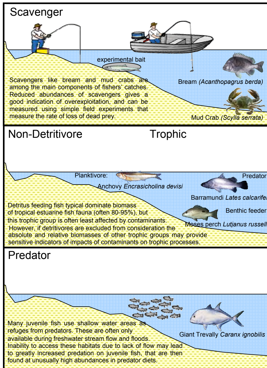
Figure 3: Three examples of simple biological indices with the potential to provide information on impacts crucial to ecological processes in tropical estuaries.
