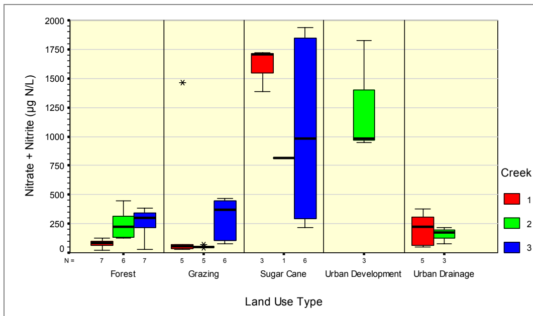
Figure 6: A boxplot showing the relative distribution of nitrate + nitrite ( \text{NO}_x ) ( \mu\text{g N/L} ) in river and creek flows for the five land use activities within the Mackay-Whitsunday region for the 2004/2005 wet season (sourced from Rohde et al. 2006a).
