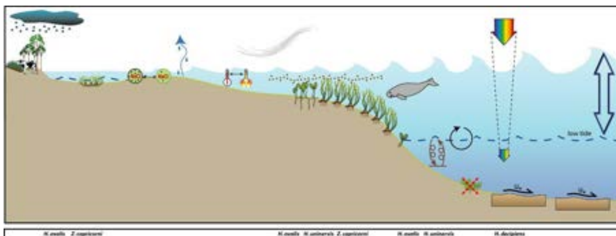
Figure 95. Conceptual diagram of coastal habitat in the Fitzroy region – major control is pulsed light, salinity and temperature extremes: general habitat, seagrass meadow processes and threats/impacts (see Figure 2 for icon explanation).
