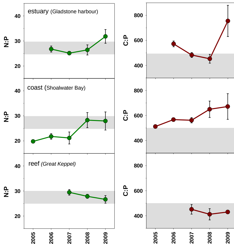
Figure 108. Elemental ratios (atomic) of seagrass leaf tissue N:P and C:P for the foundation seagrass species examined at each location in the Fitzroy region each year (species pooled) (mean \pm Standard Error). Horizontal shaded band on the N:P ratio panel represents the range of value associated with N:P balance ratio in the plant tissues. N:P ratio above this band indicates P limitation, below indicates N limitation and within indicates replete. Shaded portion on the C:P panel \leq 500 represents the value associated with C:P balance ratio in the plant tissues, C:P values < 500 may indicate nutrient rich habitats (large P pool).
