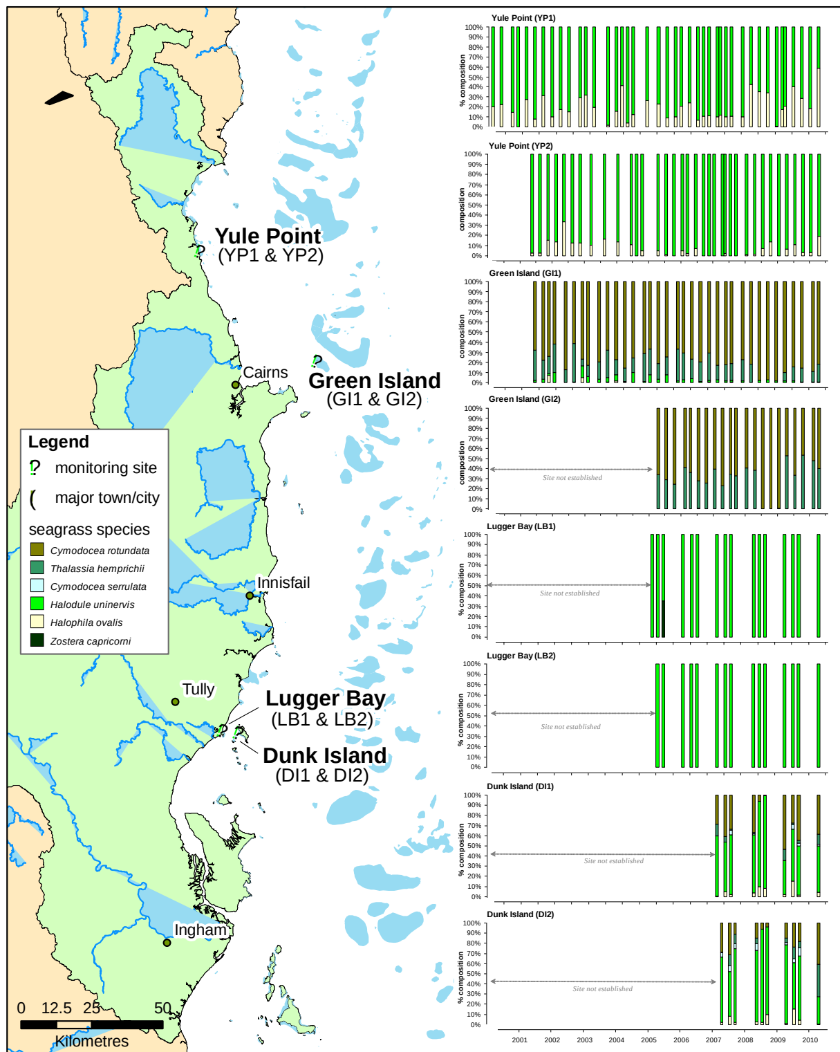
Figure 27. Location of Wet Tropics region long-term monitoring sites and seagrass species composition at each site. Please note: replicate sites within 500m of each other.
