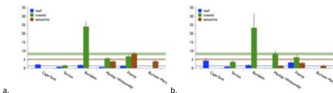
Figure 5. Reproductive effort (mean number reproductive structures per core \pm s.e.) of intertidal seagrass meadows for each habitat type for NRM regions in the GBR sampled during dry seasons. a. reproductive effort across all years sampled (2005-2010) for each habitat type in each region. Horizontal lines depict the whole of GBR mean reproductive effort across all sampling years by way of reference. b. reproductive effort for the 2009 sample for each habitat type in each NRM. Horizontal lines depict the whole of GBR mean reproductive effort across all sampling years by way of reference.
