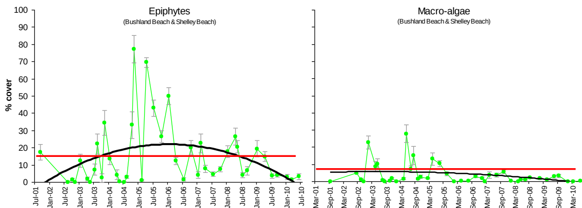
Figure 63. Mean abundance (% cover) ( \pm Standard Error) of epiphytes and macro-algae at coastal intertidal seagrass monitoring locations (sites pooled). NB: Polynomial trendline for all years pooled. Red line = GBR long-term average.
