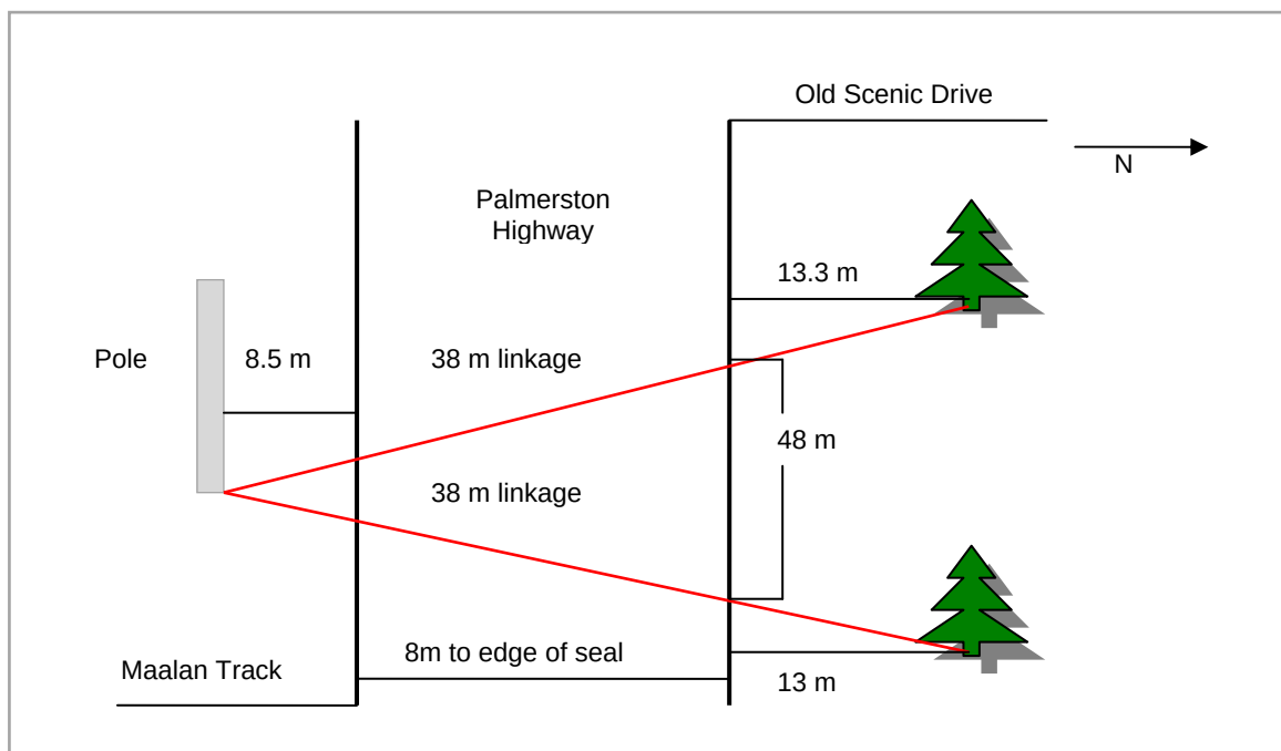
Figure 1.9 Overpass dimensions and means of attachment – Linkages 2 and 3, between Maalan Road and Old Scenic Drive.
