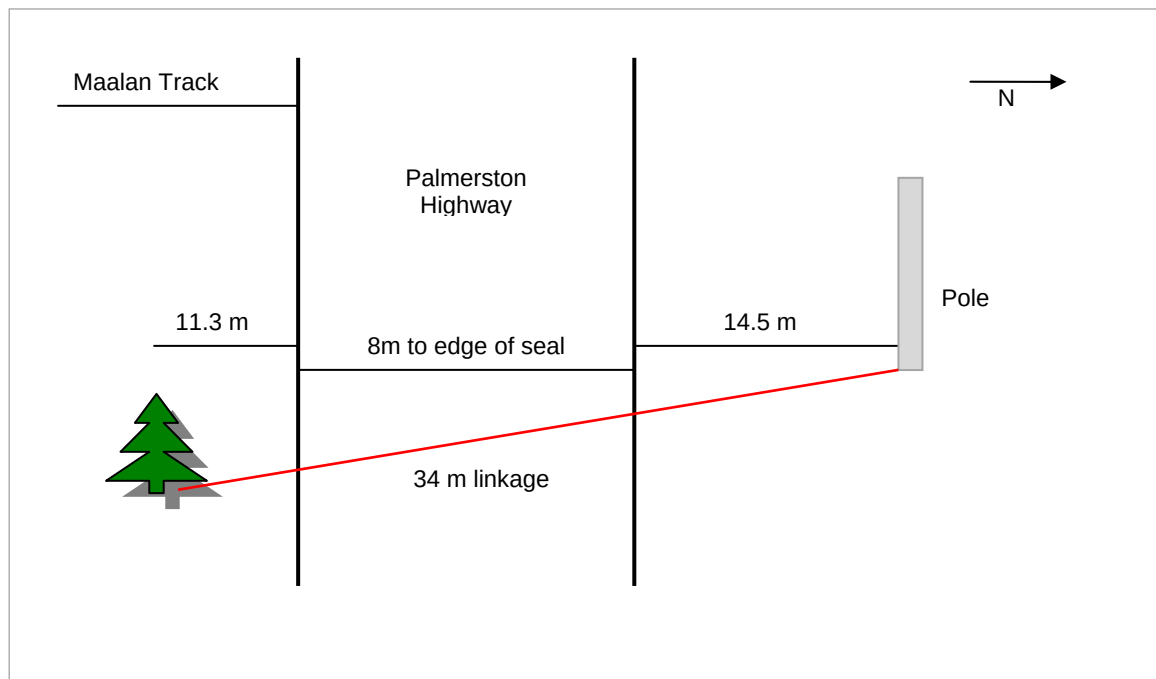
Figure 1.8 Overpass dimensions and means of attachment – Linkage 1.
