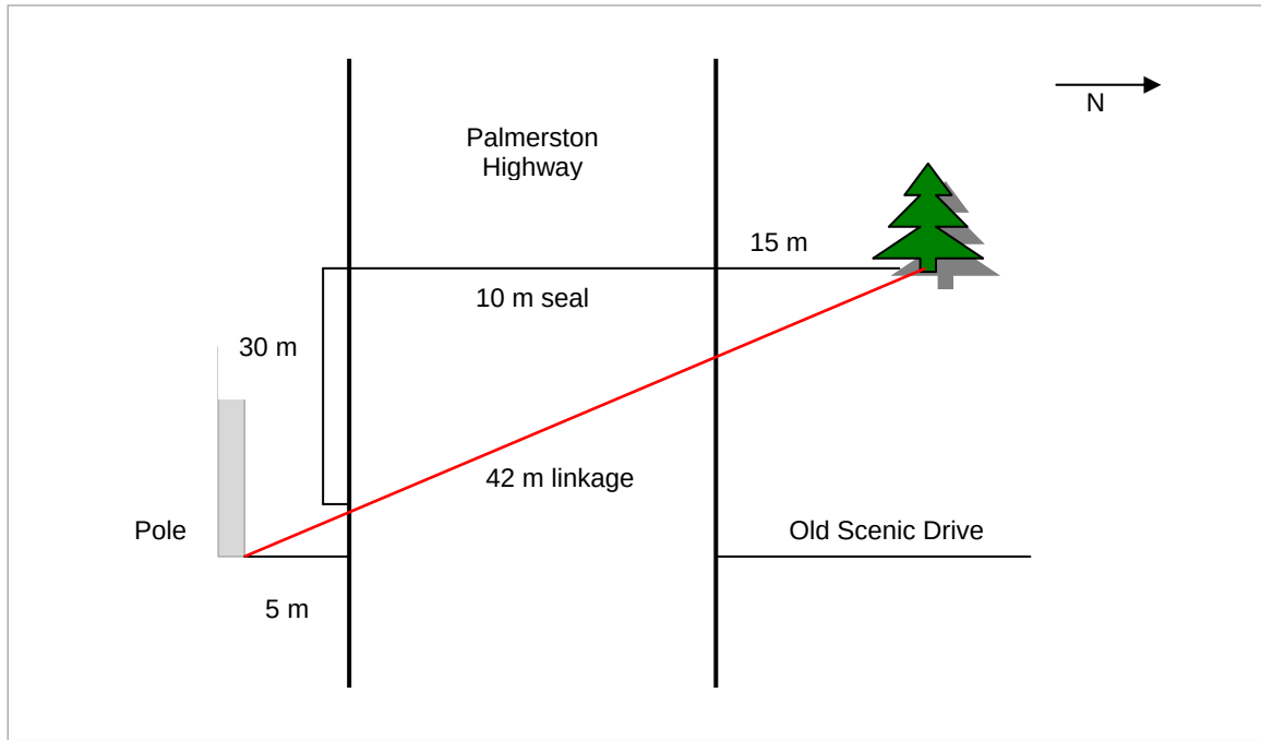
Figure 1.10 Overpass dimensions and means of attachment – Linkage 4, Millaa Millaa side of Old Scenic Drive.
