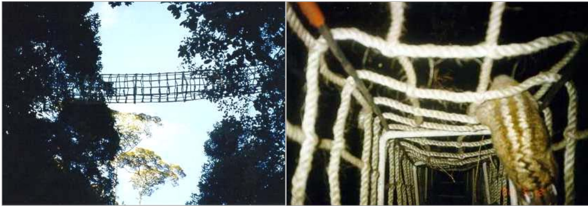
Figure 2.1 (Left) Initial rope tunnel design by Rupert Russell of the Queensland Environmental Protection Agency, installed across a forestry road in the Lamb Range area, with (right) a Green Ringtail possum making use of it. Photos courtesy of Nigel Weston.
