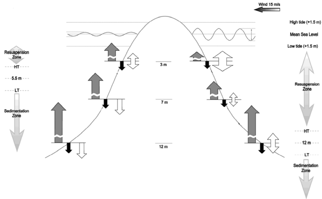
Figure A4: Schematic representation of the observed fine sediment budget at High Island, northern GBR. The windward side is to the right, the lee side to the left. Black downward arrows = sedimentation rates ( \text{mg cm}^{-2} \text{d}^{-1} ) in calm weather. Dark grey upward arrows = potentially resuspendable fine sediment ( 1000 \times \text{mg cm}^{-2} ). White arrows, pointing downward if only sedimentation occurs; both upward and downward if resuspension also occurs = storm sedimentation/resuspension rates. Wave characteristics, and the resuspension and sedimentation zones at high tide (HT) and low tide (LT) are also shown. Modified from Wolanski et al. (2005).
