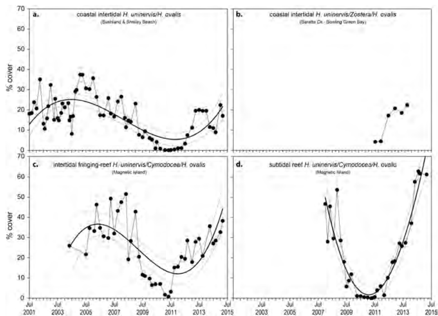
Figure 2: Seagrass abundance at Burdekin NRM region sites from 2001 to 2015, highlighting trends in abundance at Magnetic Island intertidal (c), and subtidal (d), which has undergone loss and recovery since carbohydrate collection, began in 2008 (From McKenzie et al, 2016)
