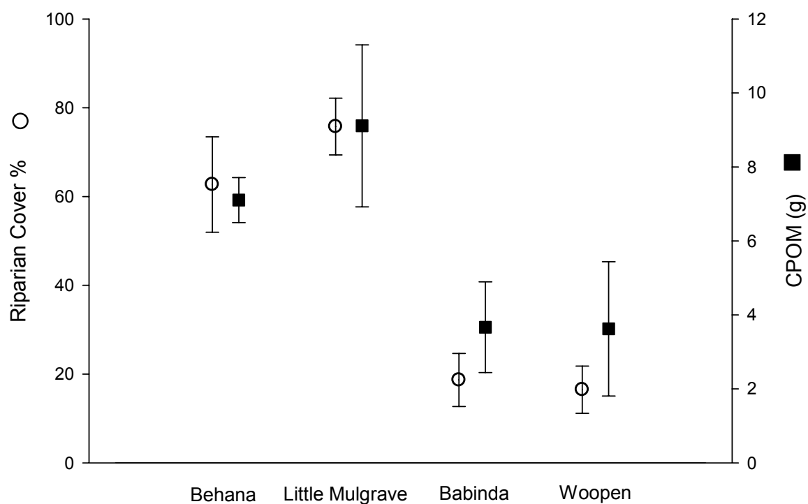
Figure 4.12. Mean % riparian cover and mean dry weight of coarse particulate organic matter (CPOM) collected in macroinvertebrate samples for each of the four streams. Error bars represent the standard errors of the means. The upper two sites are omitted from each stream because they were within Wooroonooran National Park and therefore upstream of agricultural land use.
