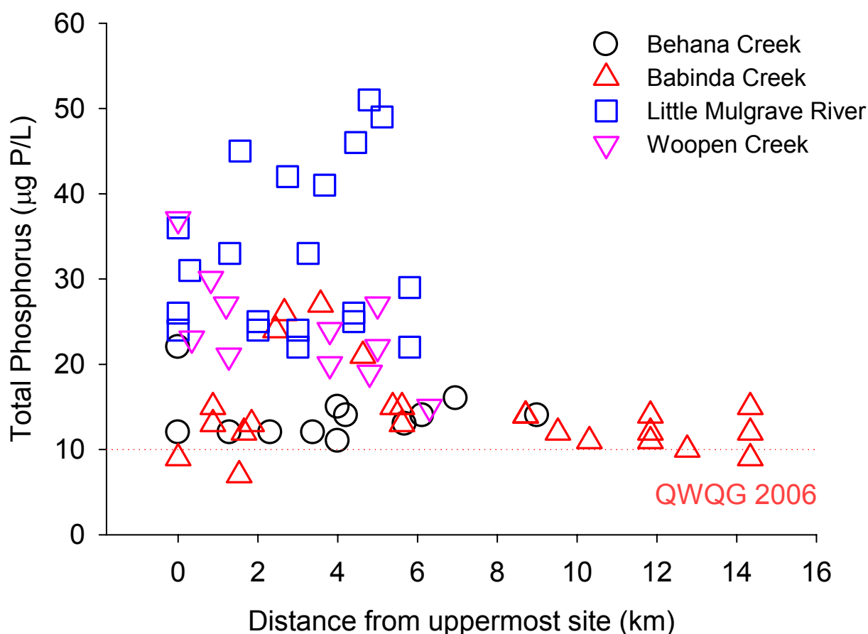
Figure 2.45. Total phosphorus concentrations in the four study streams. The horizontal line represents the Queensland Water Quality Guideline (2006) concentrations.
