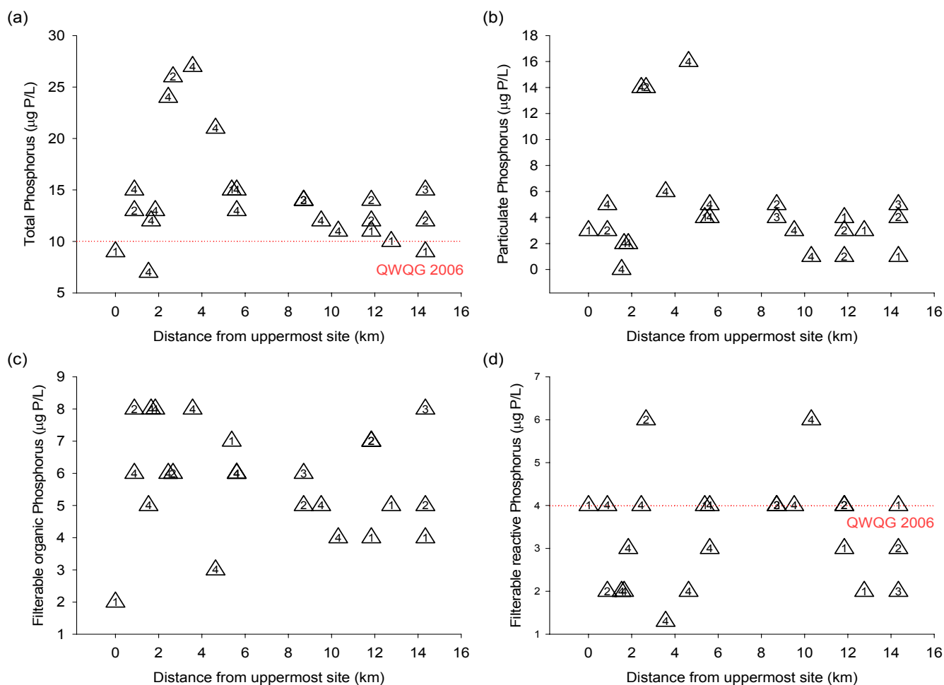
Figure 2.42. Phosphorus values measured in Babinda Creek: (a) total phosphorus, (b) particulate phosphorus, (c) filterable organic phosphorus, (d) filterable reactive phosphorus. Numbers indicate sample series described in Table 2.7. The horizontal lines represent the Queensland Water Quality Guideline (2006) concentrations.
