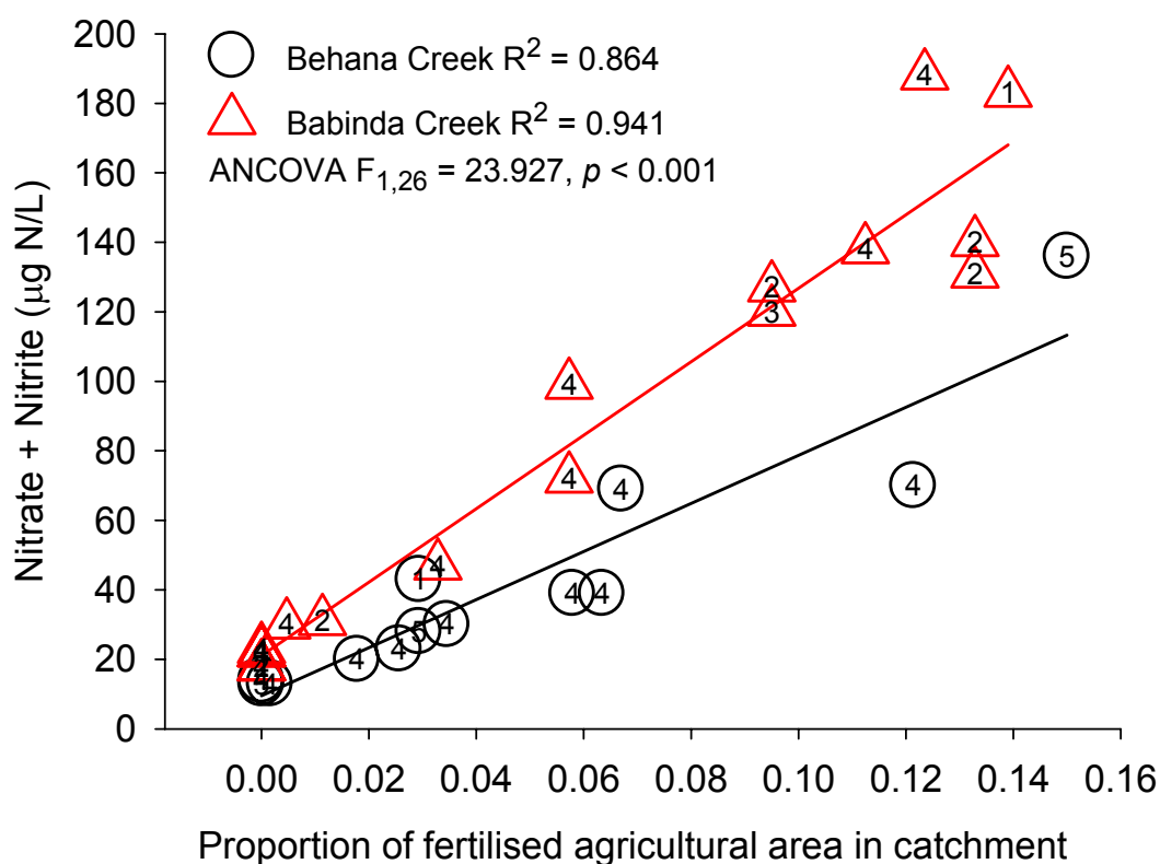
Figure 2.37. Relationship between concentration of nitrate + nitrite ( \text{NO}_x ) at sites along Behana and Babinda Creeks and the proportion of the catchment area currently used for agriculture. Regressions are based on the linear equation y_1 = y_0 + a(x) . The significant difference between streams is shown by the results of an analysis of covariance (ANCOVA) using the proportion of agricultural area in catchment as a covariate.
