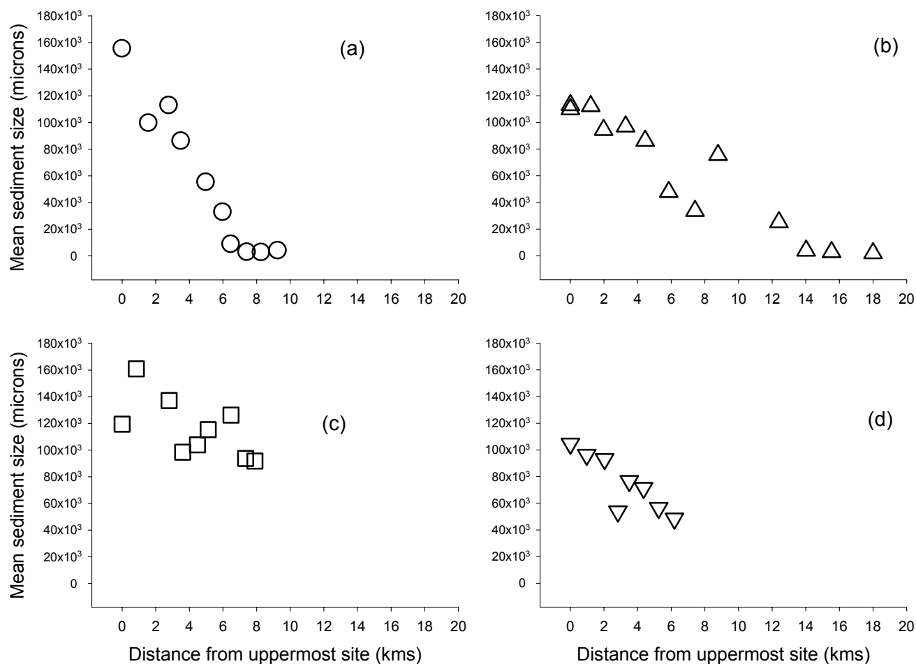
Figure 4.1. The mean substratum particle sizes recorded at sample sites in relation to the distance from the uppermost site, positioned at the base of the range, for each of the four streams surveyed: (a) Behana Creek (b) Babinda Creek (c) Little Mulgrave River (d) Woopen Creek.
