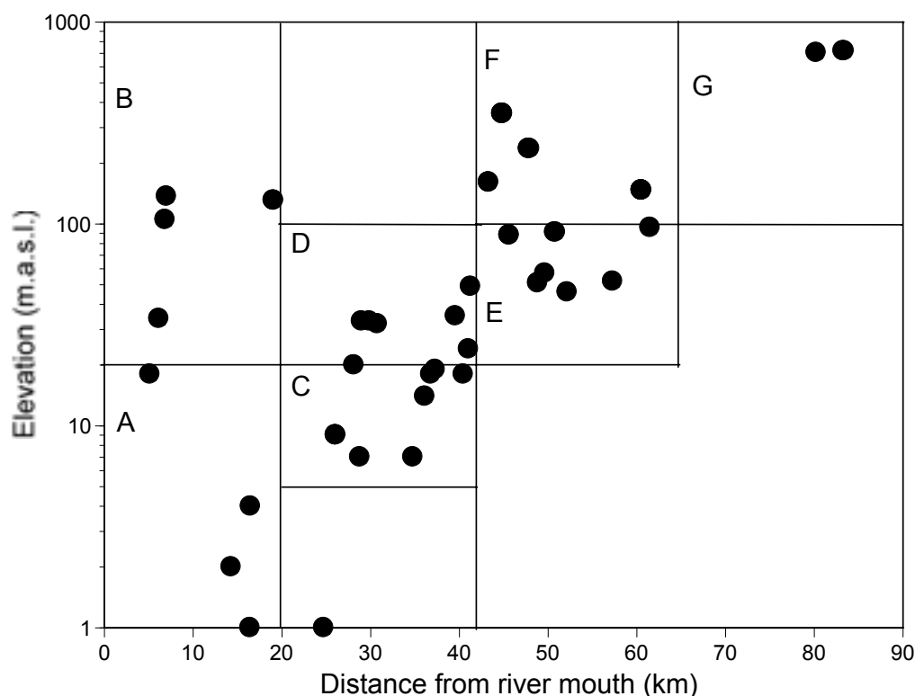
Figure 5.4. The position of reference sites within the riverine landscape as determined by elevation and distance upstream from the river mouth. Note that the some sites situated close to one another are obscured on the figure. The lines on the figure denote sites groups defined on the basis of similarities in proximity to the river mouth and elevation. Sample size for each group is given in Table 7.8.
