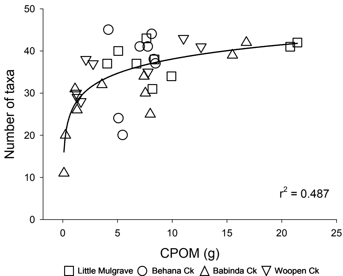
Figure 4.16. The relationship between coarse particulate organic matter (CPOM) collected in macroinvertebrate samples and the number of macroinvertebrate taxa for each of the four streams. Regression is based on the equation y_1 = y_0 + a \cdot \ln(x) .
