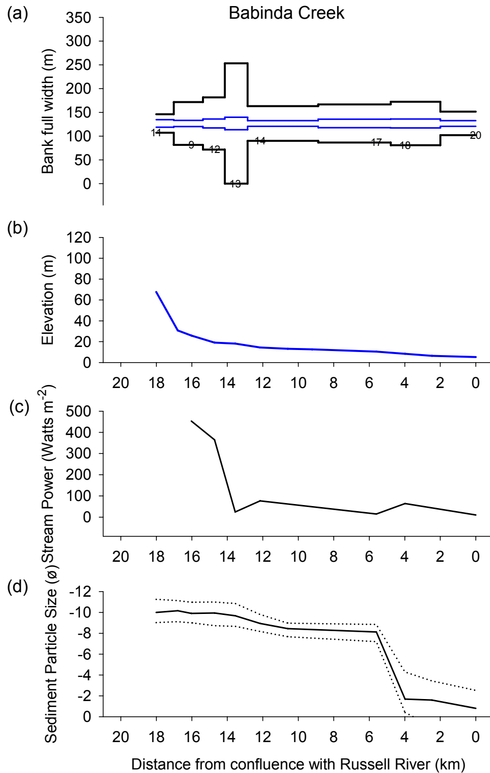
Figure 2.16. Longitudinal patterns of geomorphic and hydraulic attributes of Babinda Creek: (a) bank-full width, (b) elevation, (c) stream power and (d) median ( d_{50} ), d_{10} and d_{90} sediment particle sizes.
