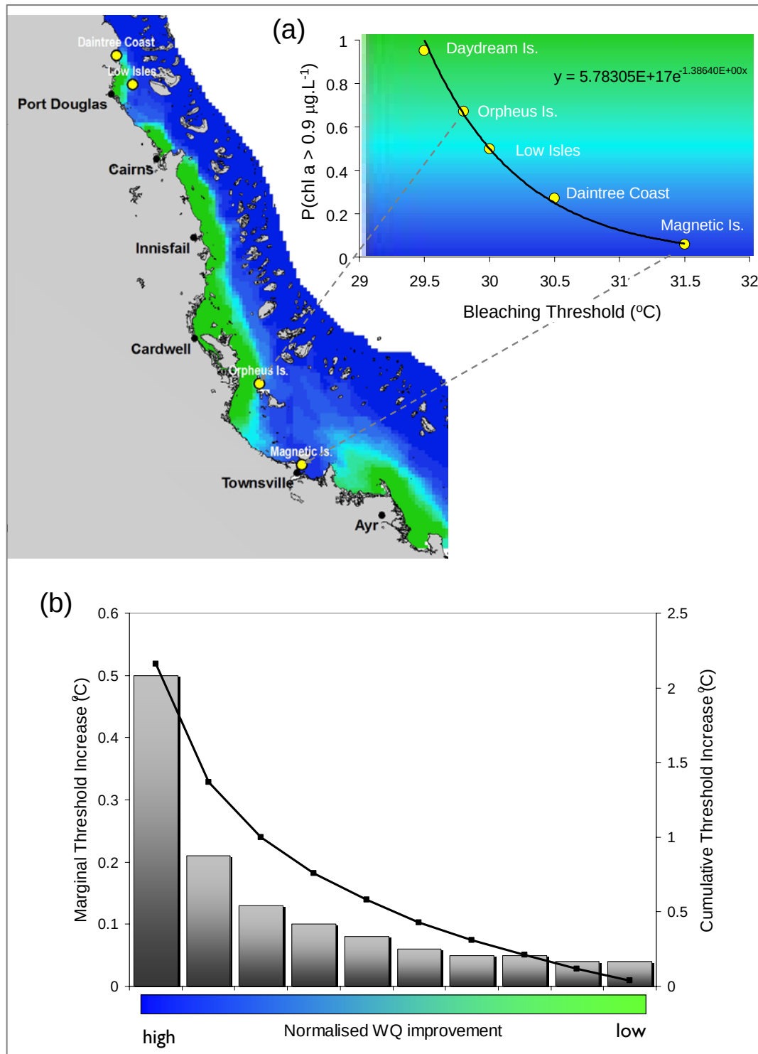
Figure 1: (a) Quantitative linkage between upper thermal bleaching limits ( ^{\circ}\text{C} ) and the degree of exposure to nutrient enriched terrestrial waters. Coastal reef waters with high DIN-enriching impact are characterised by a higher annual exceedence probability (AEP) of Chl a > 0.9 \mu\text{g.L}^{-1} . (b) Marginal (bar) and cumulative (line) increase in coral bleaching threshold ( ^{\circ}\text{C} ) across the (normalised) inshore DIN-enrichment gradient. The relationship links the greatest opportunity for improvement with the highest levels of terrestrial water quality improvement.
