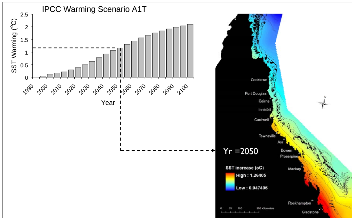
Figure 2: Spatial and temporal predictions of the increase in summer maximum SST (°C) resulting from the IPCC warming scenario A1T.
