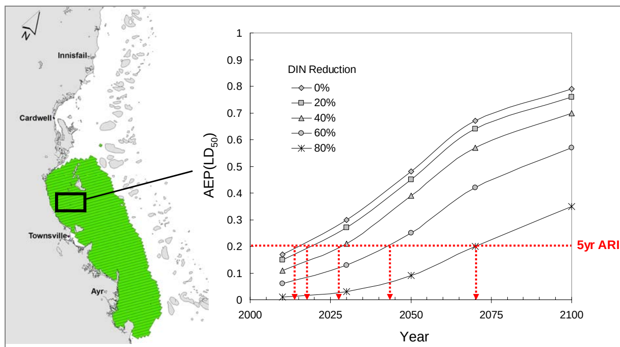
Figure 6: Projected AEP of LD 50 mortality events given a 20%, 40%, 60% and 80% reduction in end-of-river DIN concentration. The five-year ARI (red line) is indicative of the maximum bleaching disturbance frequency for the continued maintenance of a hard coral-dominated reefscape on the GBR.
