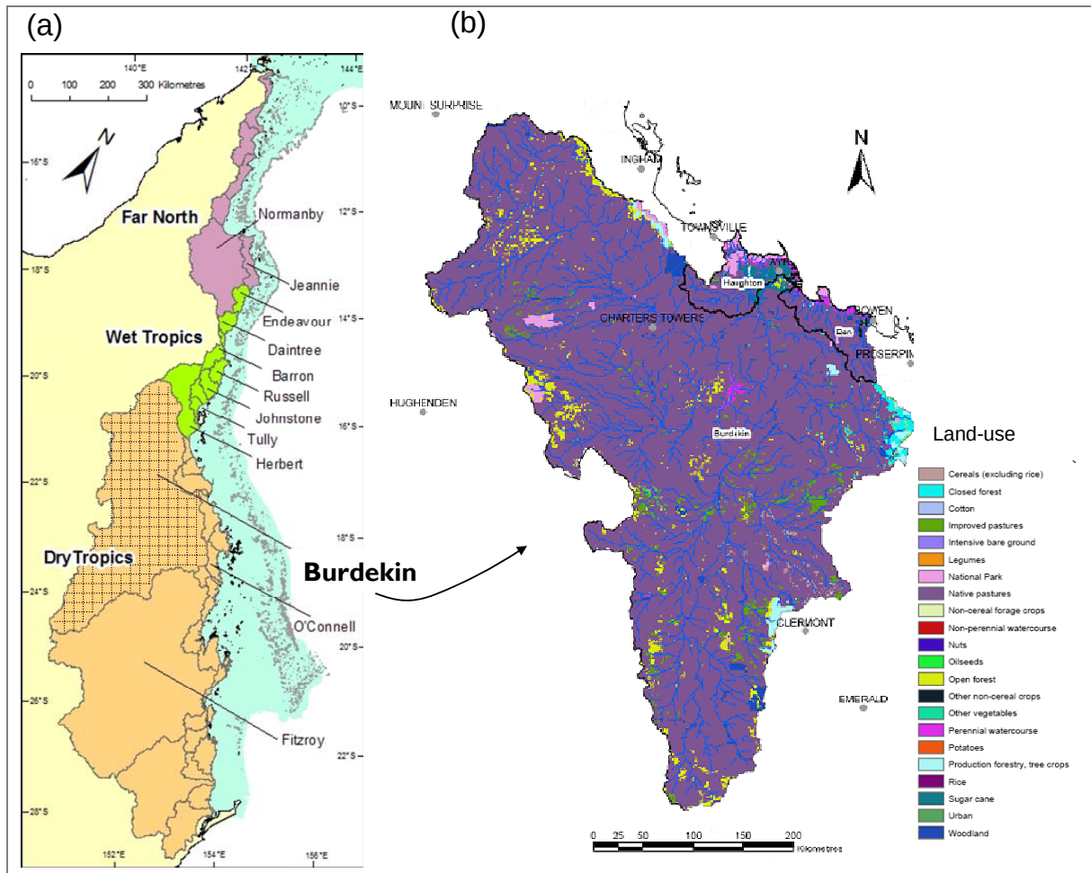
Figure 3: (a) The Great Barrier Reef and its catchments. (b) Land use in the Burdekin River catchment.
