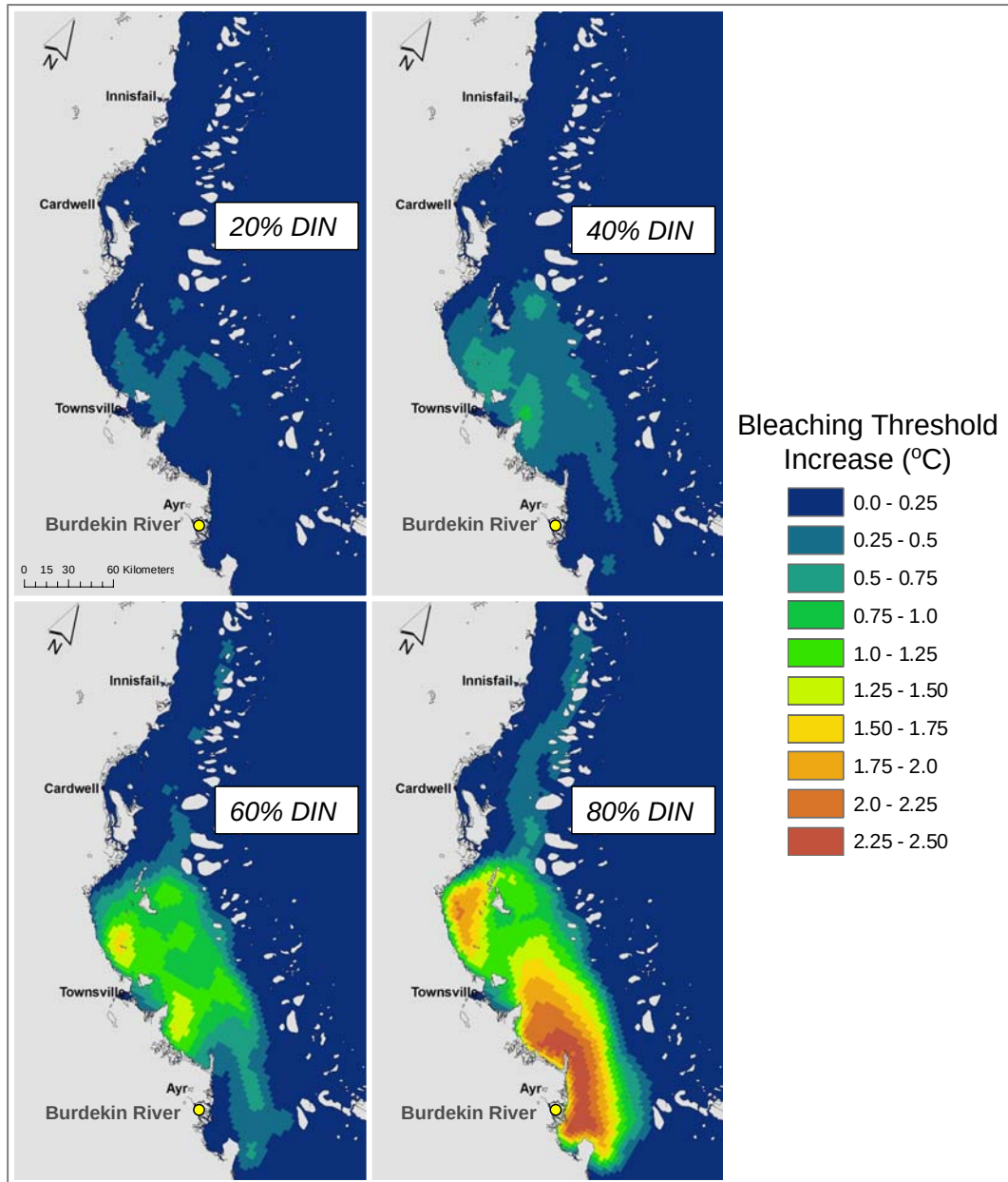
Figure 5: Modelled improvement in upper thermal bleaching threshold (°C) due to a 20%, 40%, 60% and 80% reduction in end-of-river DIN concentration for the Burdekin River catchment.
