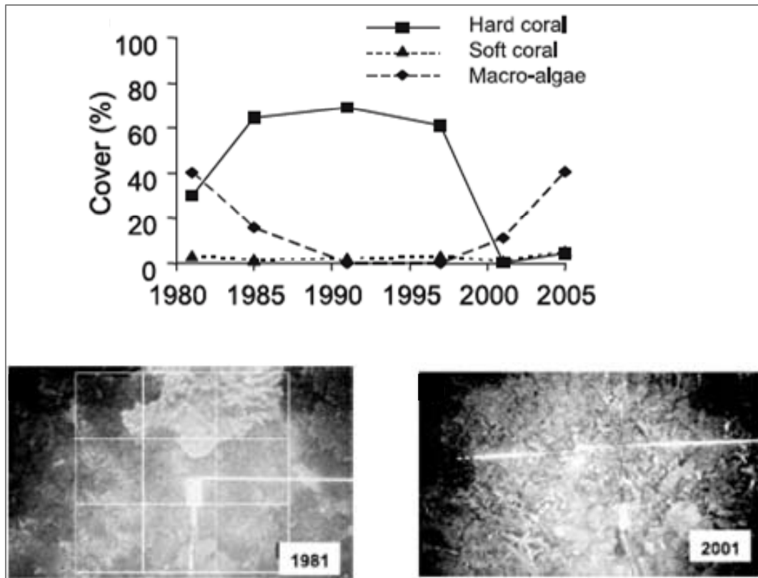
Figure 4: Photo-transect of the shallow fore-reef zone of Pandora Reef detailing the trajectory of hard coral, soft coral and macro-algae cover (percent) during the period 1981-2005 (after Done et al. 2008). The significant loss of coral cover due to the 1998 GBR bleaching event has been slow to recover due to the subsequent bleaching event in 2002.
