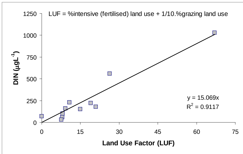
Figure 6: DIN export concentrations as a function of the proportion of fertilised land-use (LUF) in selected GBR catchments (after Wooldridge et al. 2006). The assumption that grazing lands contribute only one-tenth of the DIN export per area compared to fertilised cropping lands is based on a number of comparison studies summarised in Brodie and Mitchell (2005).
