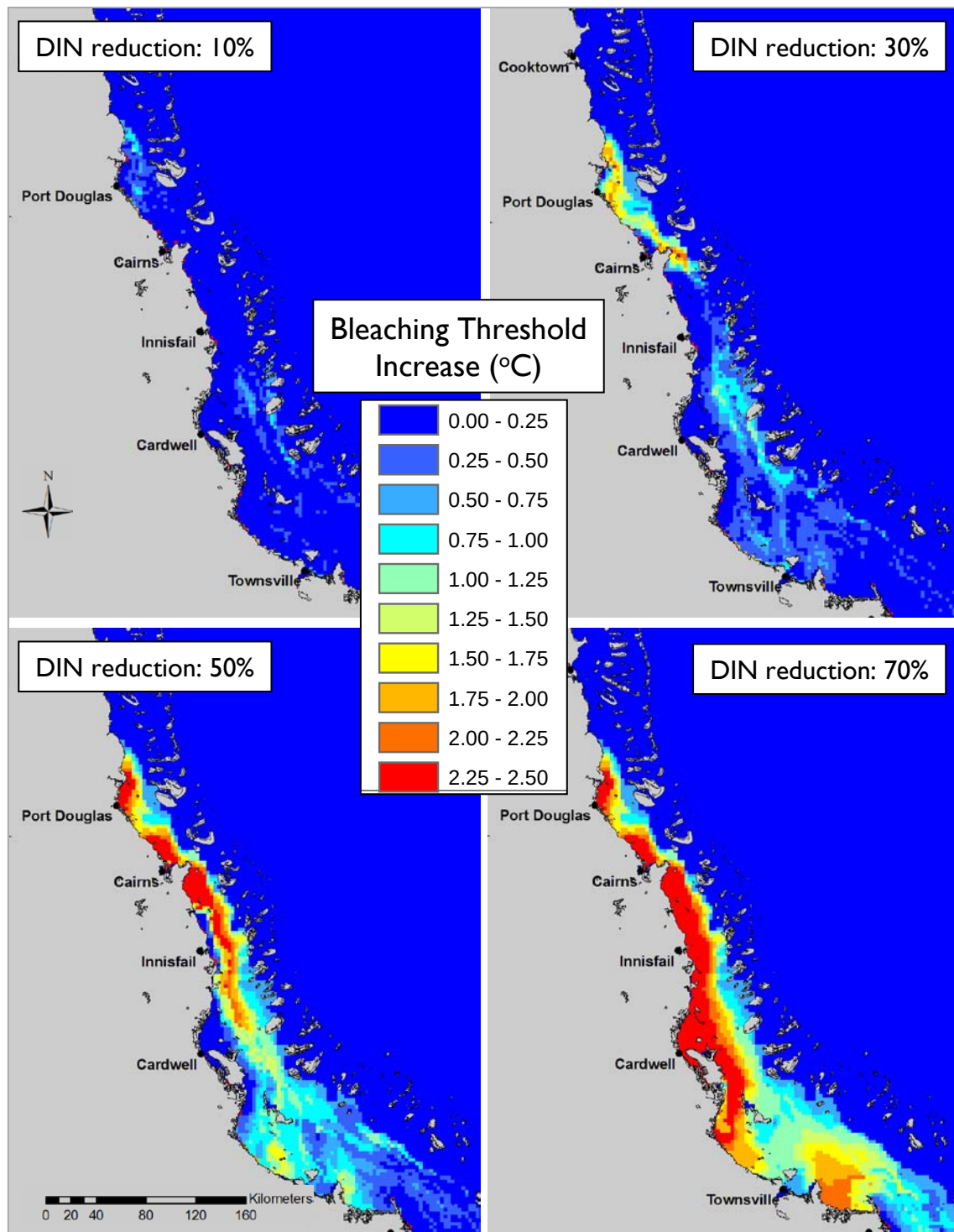
Figure 10: Simulated increased in the upper thermal bleaching limits (°C) of inshore corals due to specified (uniform percentage) reductions in end-of-river DIN loading for the numerous basins that drain the GBR catchment.
