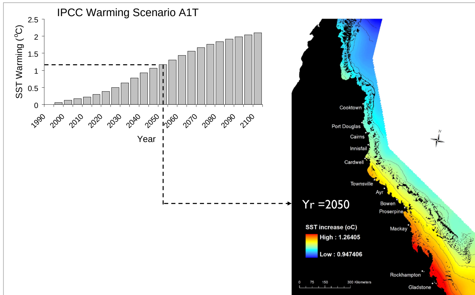
Figure 1: Predicted increase in SST (°C) for the Great Barrier Reef in response to a 'mid-range' IPCC warming scenario.
