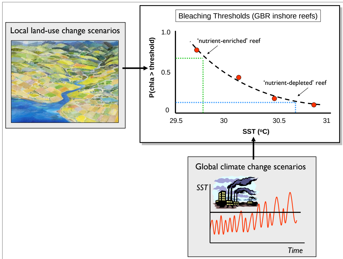
Figure 5: Conceptual modelling framework that enables the impact of 'local' (viz. water quality) and 'global' (viz. \text{CO}_2 / temperature reduction) management strategies to be assessed in terms of their joint (conditional) potential to reduce the future likelihood of mass coral bleaching on the Great Barrier Reef.
