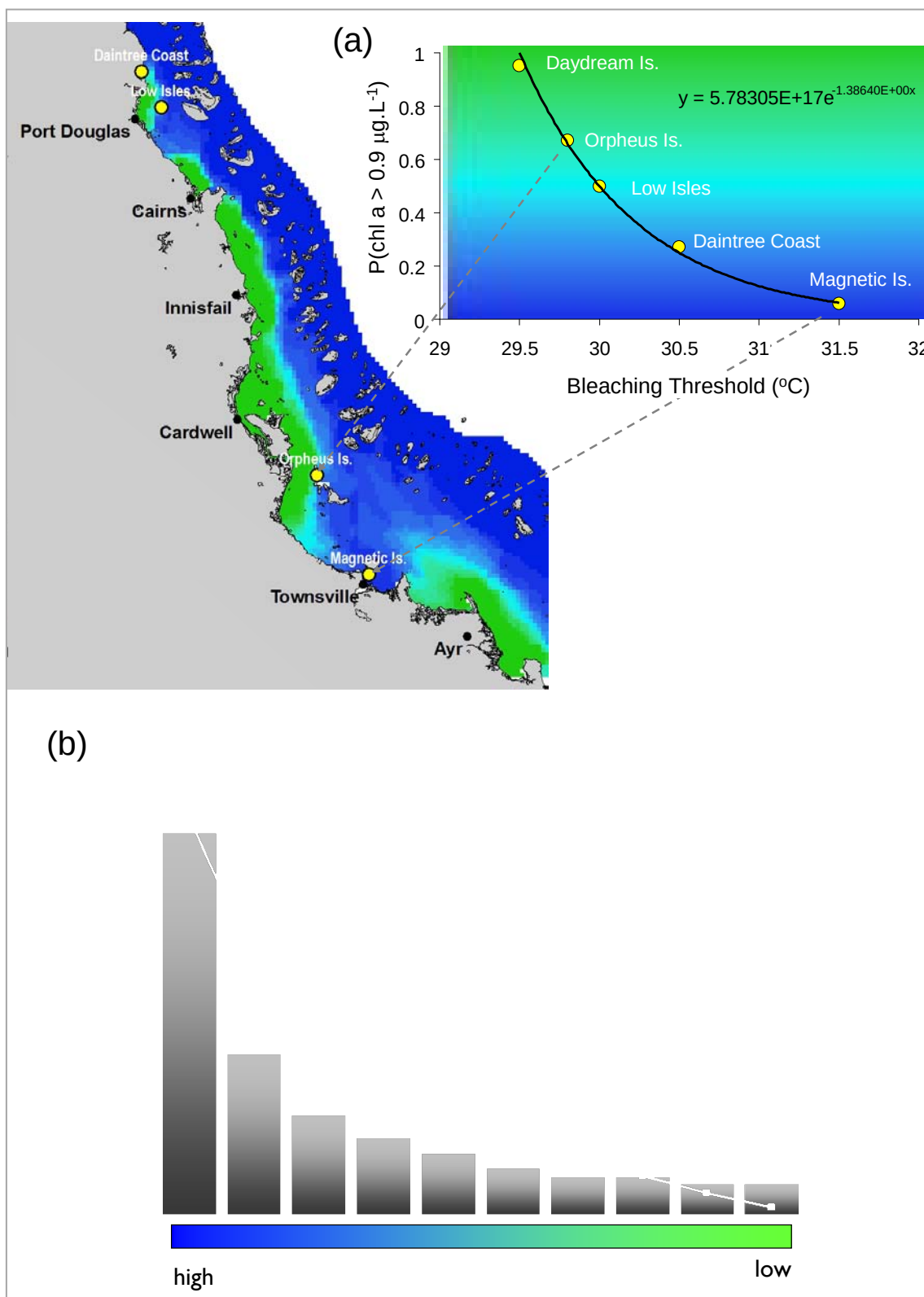
Figure 4: (a) Quantitative linkage between upper thermal bleaching limits (°C) and the degree of exposure to nutrient enriched terrestrial waters. Coastal reef waters with high DIN-enriching impact are characterised by a higher annual exceedence probability (AEP) of [Chl a ] > 0.9 \mu\text{g L}^{-1} . (b) Marginal (bar) and cumulative (line) increase in coral bleaching threshold (°C) across the (normalised) inshore DIN-enrichment gradient. The relationship links the greatest opportunity for improvement with the highest levels of terrestrial water quality improvement.
