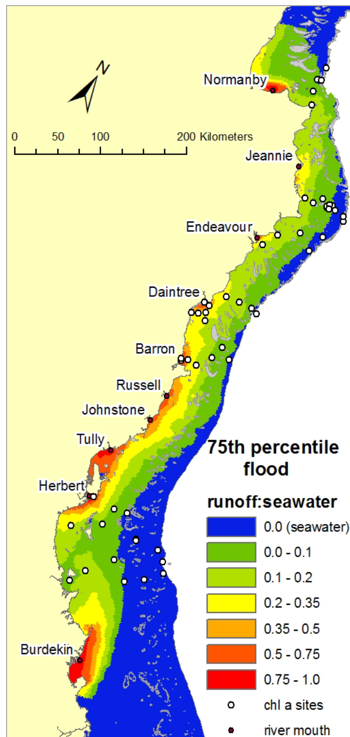
Figure 8: Flood plume (runoff:seawater) dilution rates within the GBR lagoon for a 75 th percentile flood event.
