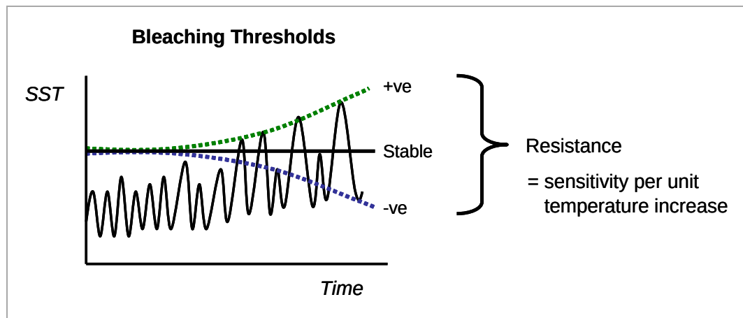
Figure 2: Schematic representation of trends in sea temperatures (solid line) and 'resistance' to coral bleaching (dotted lines). Anthropogenic pressures tend to reduce resistance through time (falling dotted line). Prospective mechanisms that could increase resistance (rising dotted line) include: (i) endosymbiont reshuffling (Berkelmans and van Oppen 2006), (ii) community composition shifts towards corals that can counter the bleaching response via access to stored tissue reserves (Loya et al. 2001) or heterotrophic energy sources (Borell and Bischof 2008), (iii) region-scale amelioration of poor water quality (Wooldridge and Done 2009; Wooldridge 2009b).
