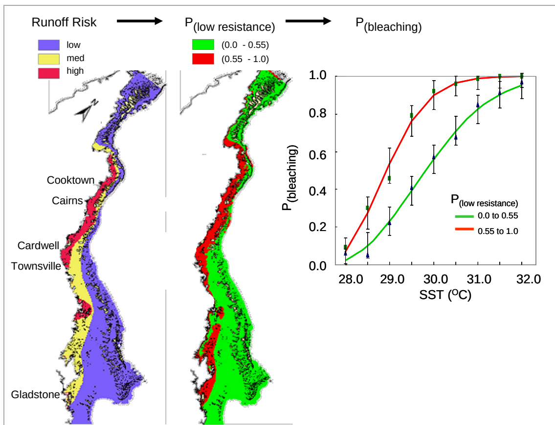
Figure 3: Regional-scale coral bleaching analysis on the GBR (after Wooldridge and Done 2009). Inshore coral reef areas with high runoff exposure risk are shown to correspond (in a probabilistic sense) with reefs that displayed a lower resistance to thermal stress (red zone) during the 1998 and 2002 mass bleaching events. Accumulated reef responses (observed) from within the low resistance (red zone) areas confirm the increased risk of bleaching (per unit increase in SST), and reflect an averaged lowering in upper thermal bleaching threshold of ~1.0-1.5°C.
