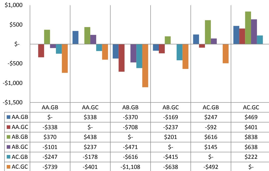
Figure 39: BDK Delta large farm NPV of changing practice ($/ha/10yr)
