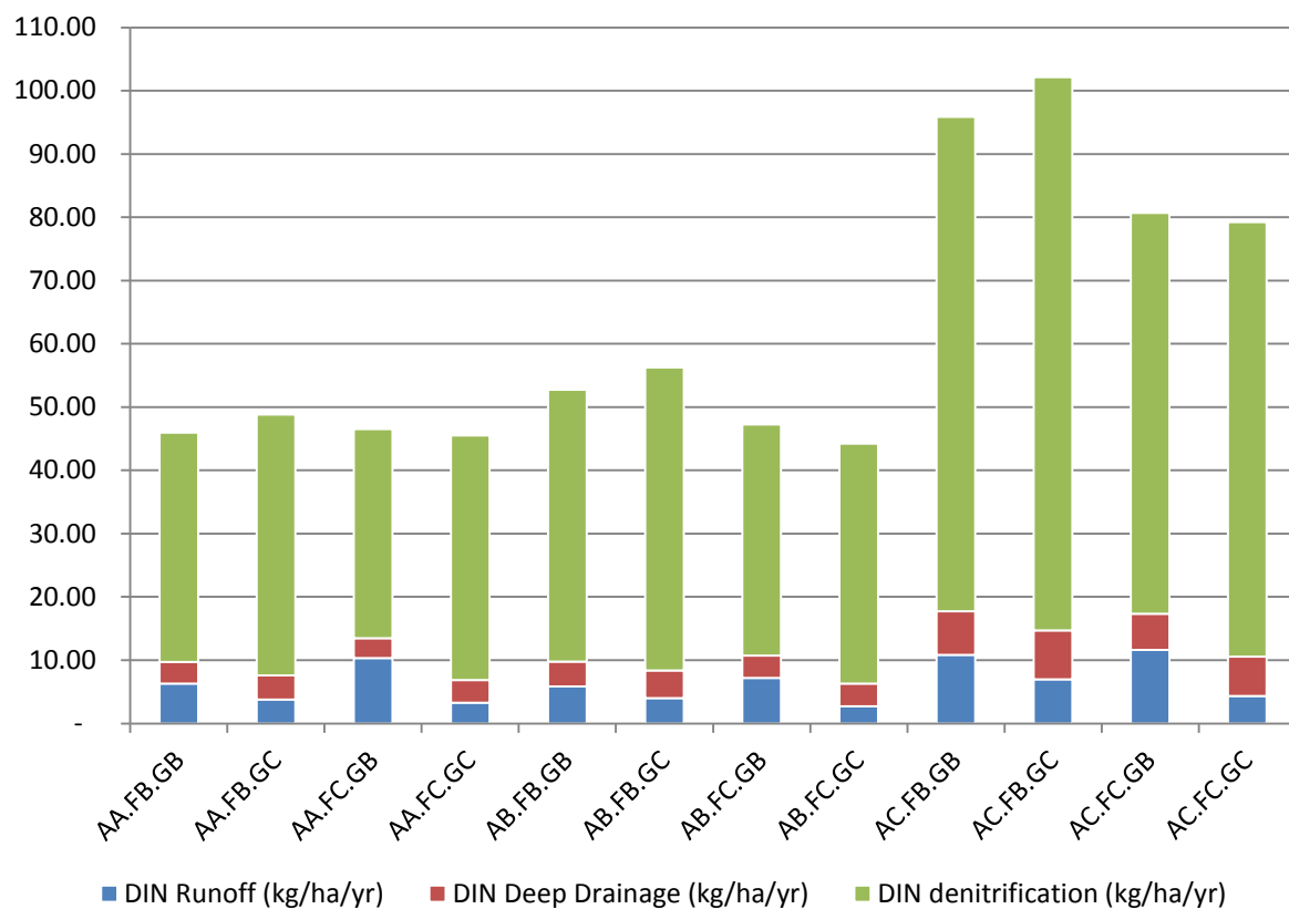
Figure 29: Burdekin River Irrigation Area N pathways (kg/ha/yr)
