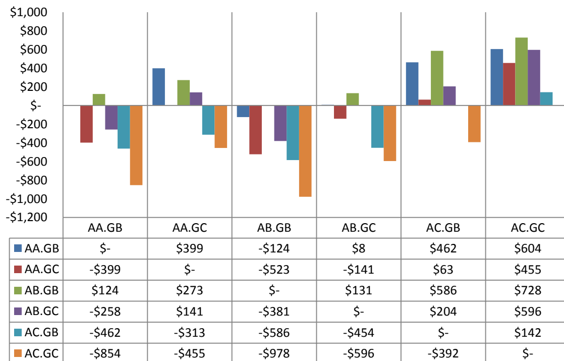
Figure 31: Mackay Whitsundays Small farm NPV of changing practice ($/ha/10yr)
