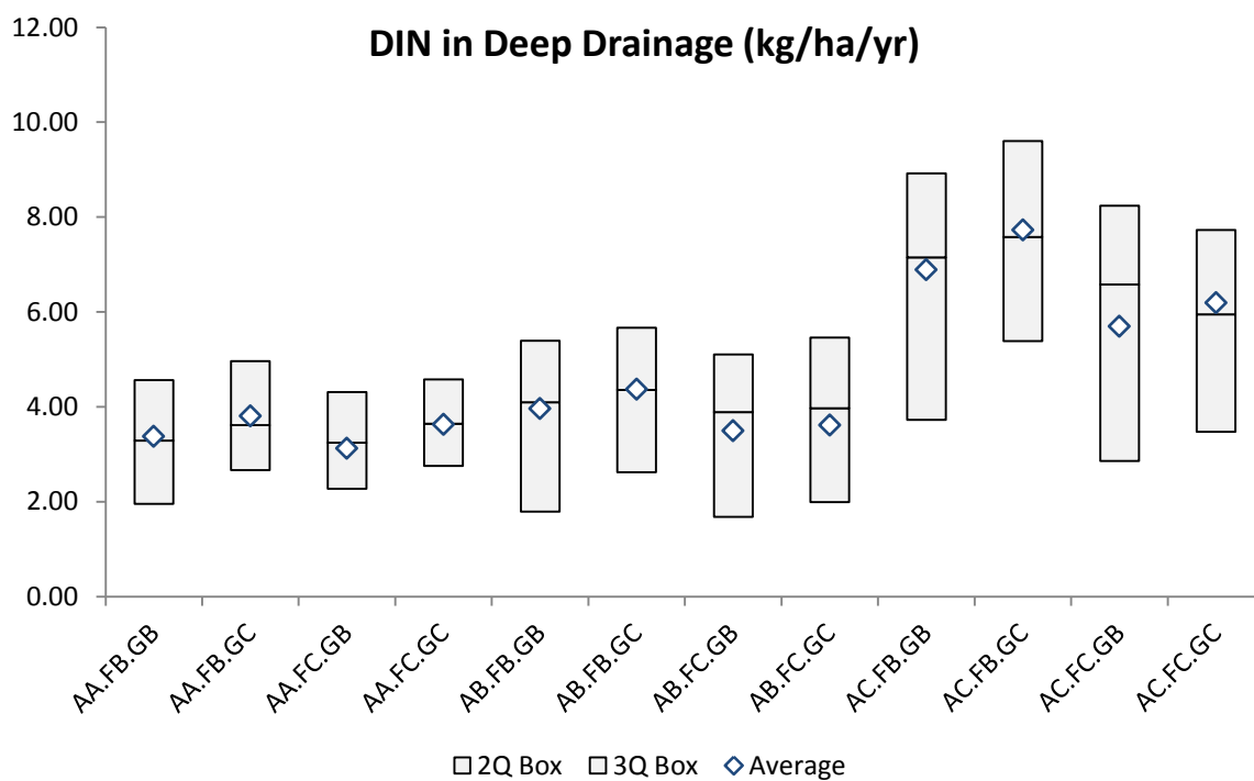
Figure 24: Burdekin River Irrigation Area DIN in Deep Drainage (kg/ha/yr)
