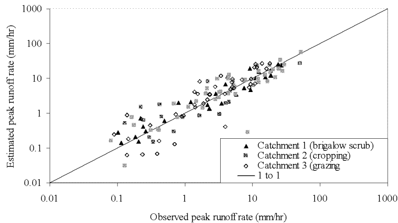
Figure 3. Observed peak runoff rate compared to the VIR method estimated peak runoff rate for the three catchments during Stage III.
