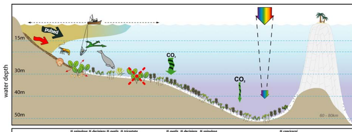
Figure 66. Conceptual diagram of deepwater habitat in the GBRWHA section of the Burnett Mary region – major control is pulsed turbidity from variable rainfall: general habitat and seagrass meadow processes (See Figure 3 for icon explanation).
