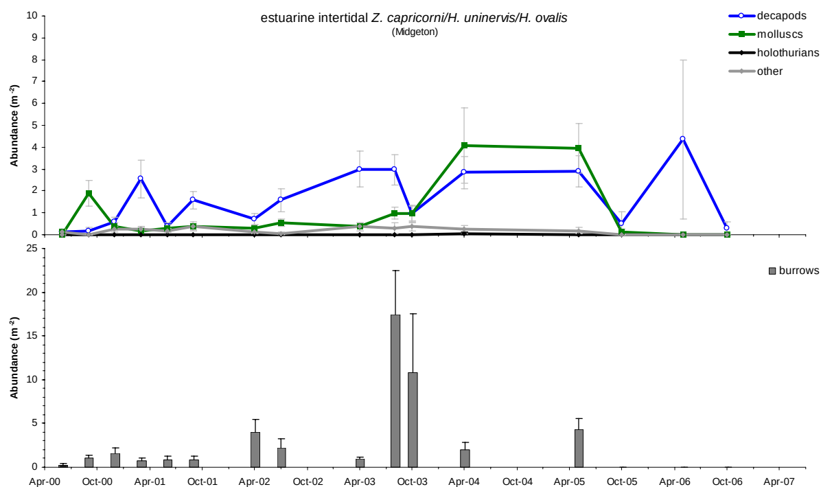
Figure 51. Abundance of associated benthic macro-fauna and bioturbation in an intertidal Zostera capricorni / Halodule uninervis / Halophila ovalis meadow in an estuary habitat over the monitoring period.
