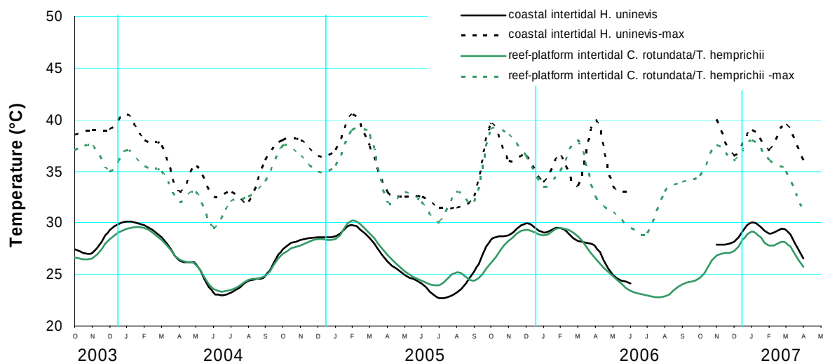
Figure 26. Within seagrass canopy temperature (°C) at intertidal meadows in a coastal and a fringing-reef habitat within the Wet Tropics region.
