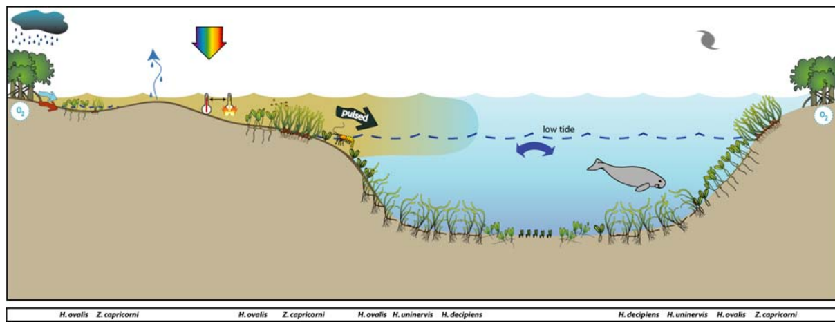
Figure 4. Conceptual diagram of estuary habitat in the Cape York region – major control is pulsed terrigenous runoff and exposure (temperature and desiccation): general habitat, seagrass meadow processes and threats/impacts (See Figure 3 for icon explanation)
