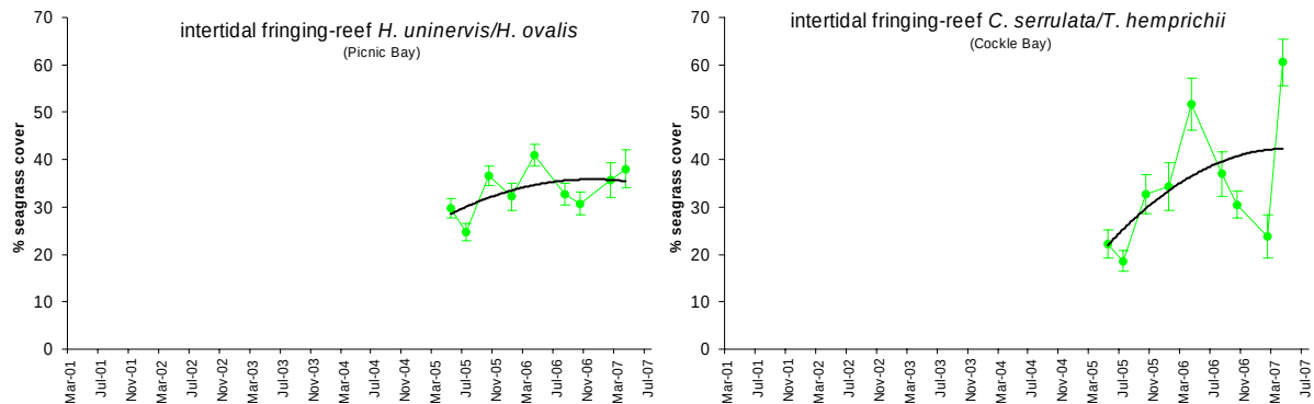
Figure 35. Change in seagrass abundance (percentage cover) at intertidal meadows on fringing reef platforms in the Burdekin Dry Tropics region.
