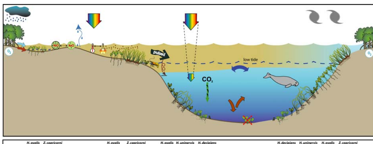
Figure 30. Conceptual diagram of Estuary habitats in the Burdekin Dry Tropics region – major control is pulsed terrigenous runoff: general habitat and seagrass meadow processes (See Figure 3 for icon explanation).
