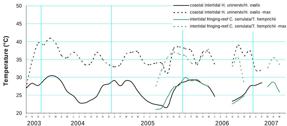
Figure 37. Within seagrass canopy temperature (°C) at intertidal meadows in a coastal and a fringing-reef habitat within the Burdekin Dry Tropics region.
