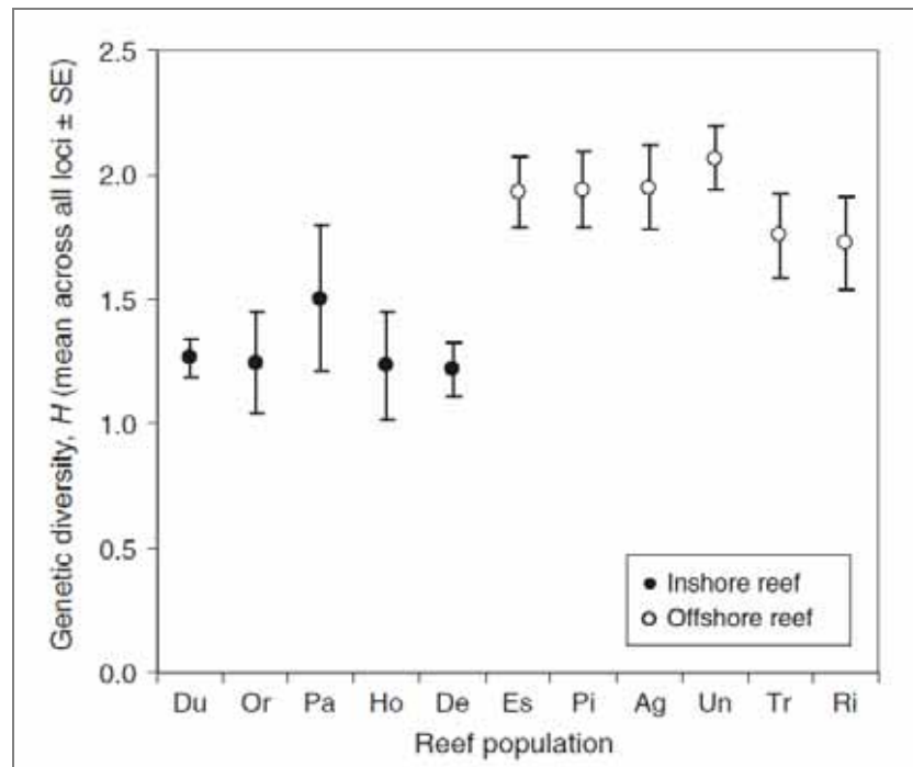
Figure 3: Genetic diversity of clade C symbionts in a widely distributed soft coral on offshore and inshore reefs of the GBR. Genetic diversity is measured by Shannon's Index (H) averaged ( \pm SE) across microsatellite loci. Abbreviated reef names: Dungeness Reef (Du), Orpheus Island (Or), Great Palm Island (Pa), Hook Island (Ho), Deloraine Island (De), Escape Reef (Es), Pickersgill Reef (Pi), Agincourt Reef (Ag), Undine Reef (Un), Trunk Reef (Tr), Rib Reef (Ri) (Howells et al. 2009).
