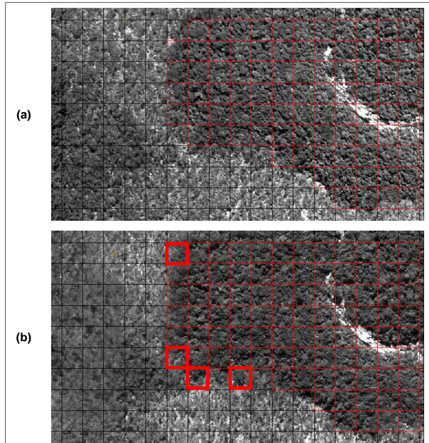
Figure 4: Illustration of change in extent of rain forest on Mount Windsor as mapped on the original 1950s orthomosaic (a) and the corresponding area in the 2008 orthomosaic (b). The 2008 orthomosaic was desaturated for comparison. Note, general vegetation thickening by 2008, including in areas of savanna vegetation. Each grid square represents a 50x50m area and the grid squares in red have been attributed for rainforest occurrence. Note the additional red grid squares (thickened borders) attributed for rainforest in the 2008 mosaic. The remaining grid squares in black represent savanna.
