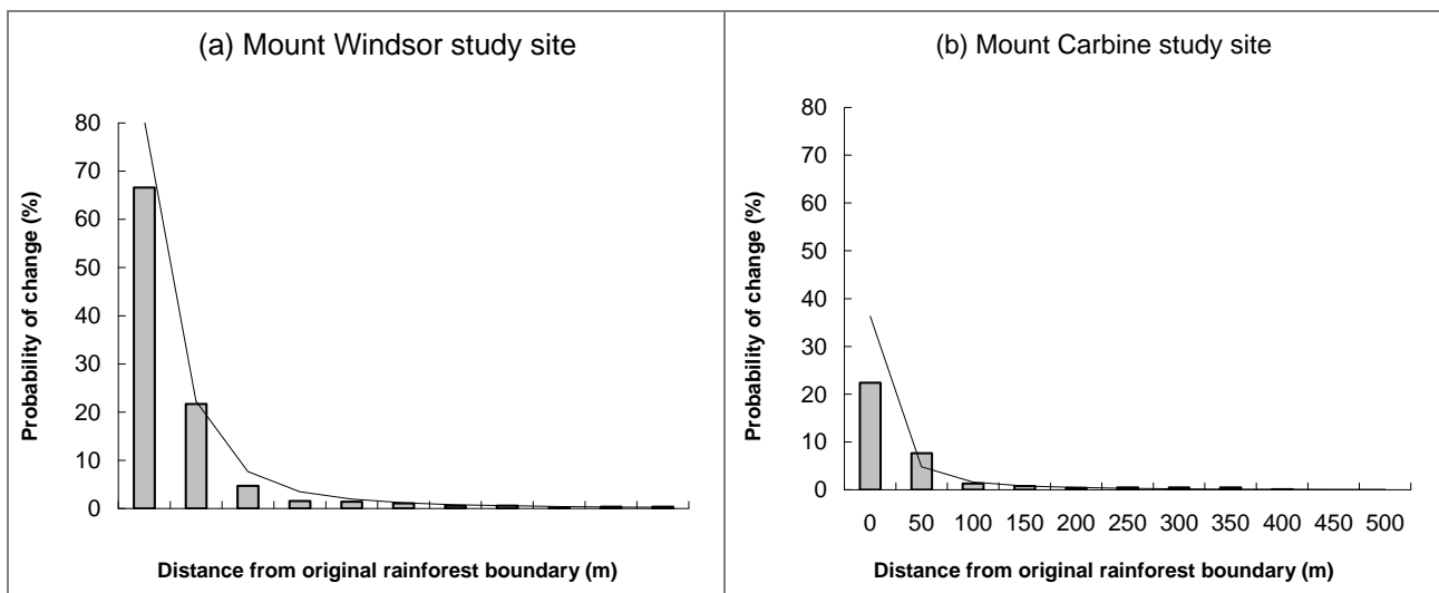
Figure 6: The observed (bars) and predicted (line) probabilities of conversion of savanna to rainforest in relation to distance to the original rainforest boundary, at the Mount Windsor (a) and Mount Carbine (b) study sites. The model predictions are based on multimodel averaging of the entire candidate set of models, weighted according to w_i and assuming mean values for all other variables.
