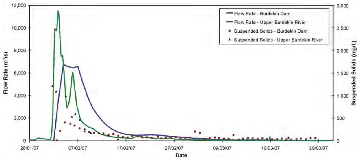
Figure 5: Flow hydrograph for the Burdekin Falls Dam overflow in the 2006/07 water year. Concentrations (in mg/L) of TSS samples collected over the flow are also shown.
