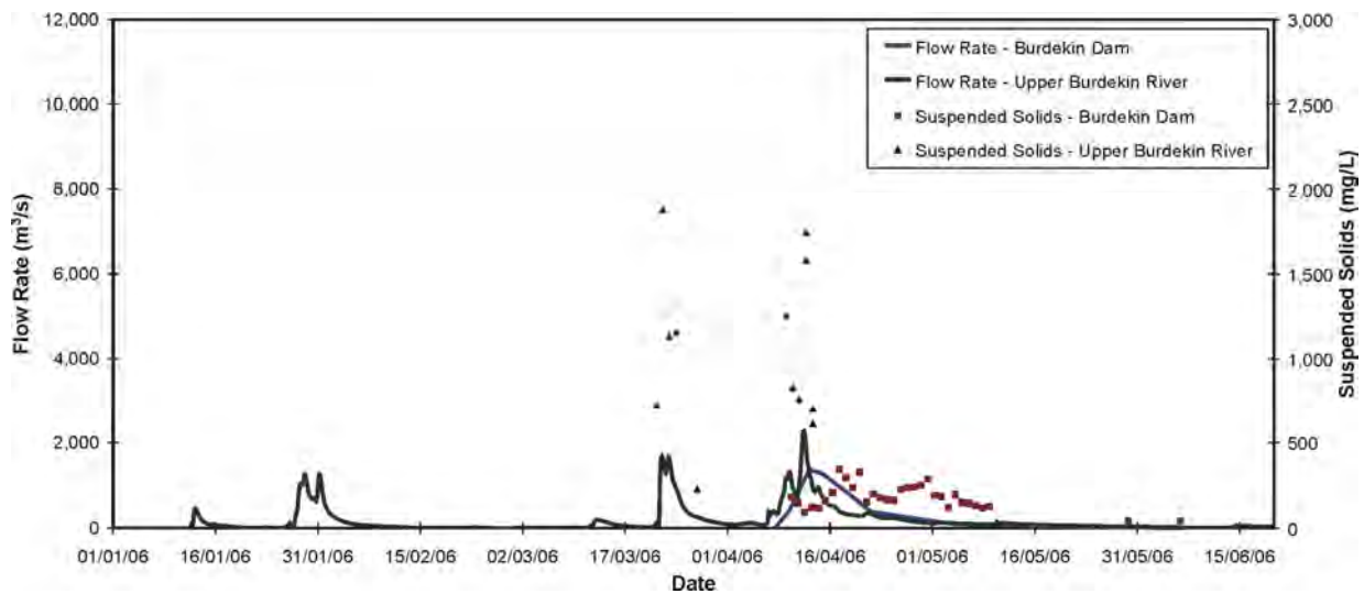
Figure 4: Flow hydrograph for the Burdekin Falls Dam overflow in the 2005/06 water year. Concentrations (in mg/L) of TSS samples collected over the flow are also shown.
