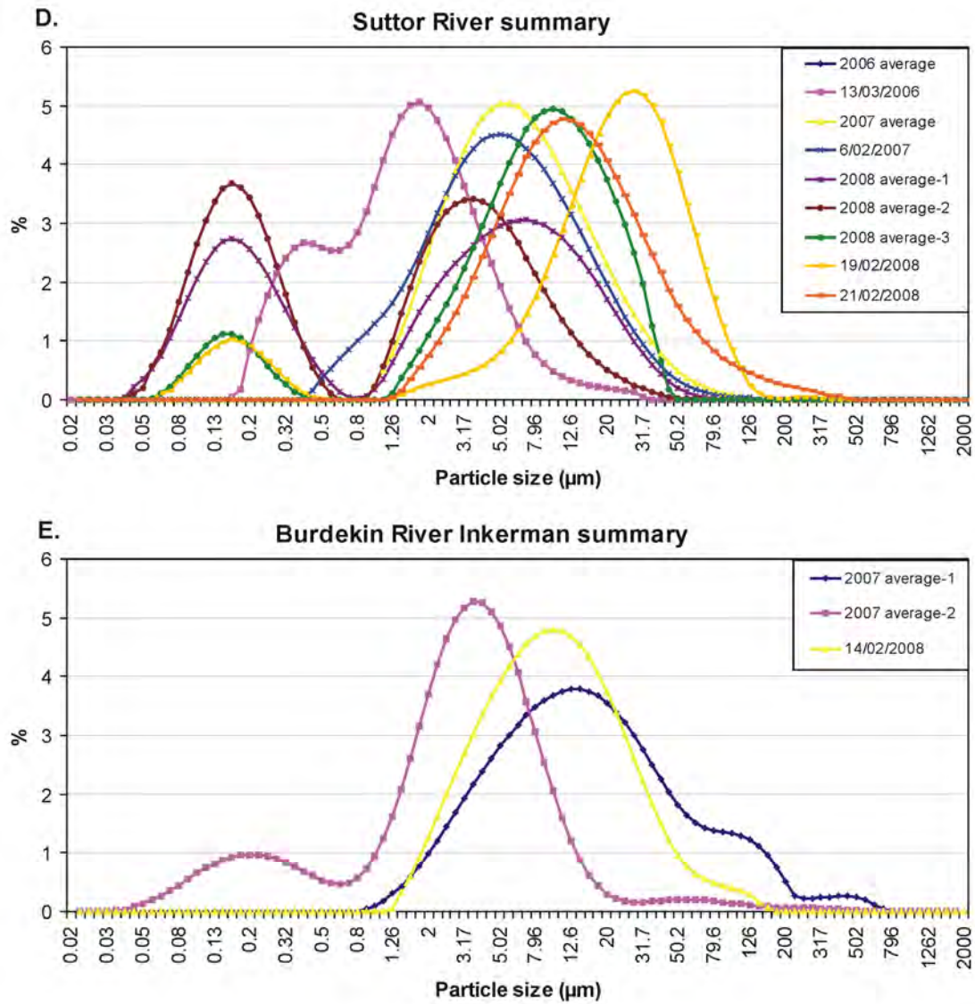
Figure 9 (continued): Particle size distributions of suspended sediment samples collected during flood events for the Suttor River (D) and Burdekin River end-of catchment (E) over the three-year monitoring period. The particle size distribution patterns that were similar have been averaged so that all distribution patterns are represented for each particular year.
