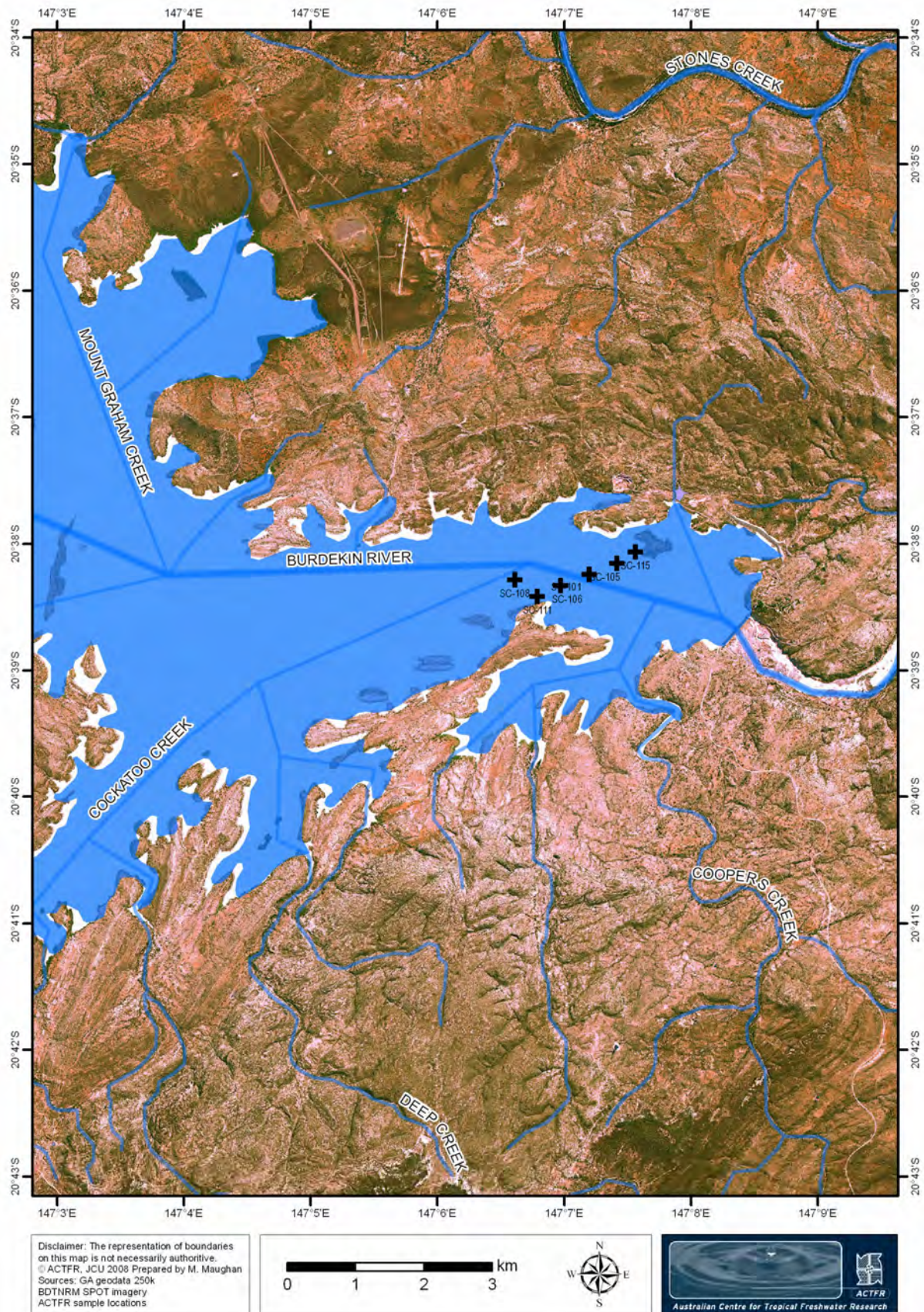
Figure 3: Suspended sediment samples were collected across the Burdekin Falls Dam reservoir on 18 January 2008 to assess the variability in concentrations across the stream profile during large flow events.
