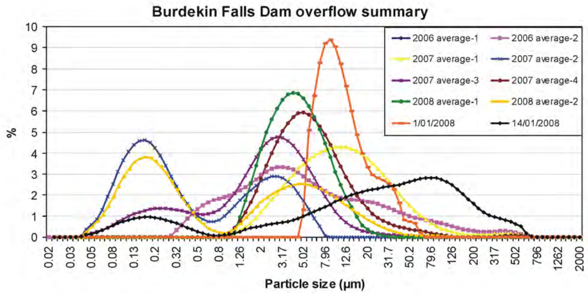
Figure 8: Particle size distributions of suspended sediment samples collected during flood events from the Burdekin Falls Dam overflow over the three-year monitoring period. The particle size distribution patterns that were similar have been averaged so that all distribution patterns are represented for each particular year.
