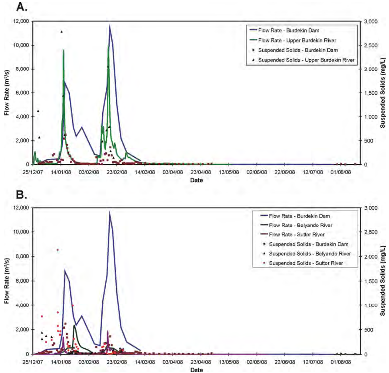
Figure 6: Flow hydrograph for the Burdekin Falls Dam overflow in the 2007/08 water year coupled with flows from the upper Burdekin River (A) and the Belyando and Suttor Rivers (B). Concentrations (in mg/L) of TSS samples collected over the flow are also shown.
