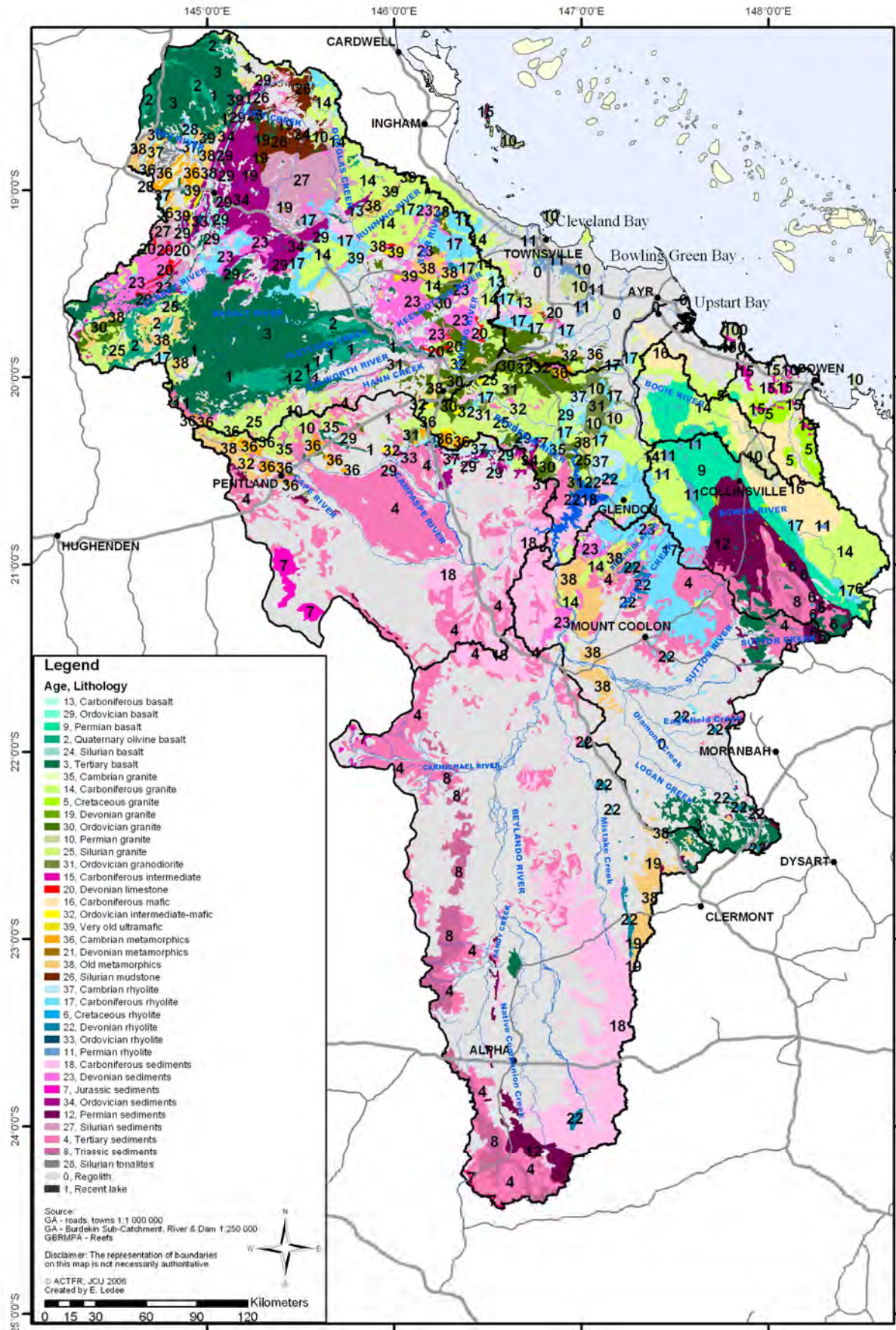
Figure 7: Geological map showing the many different rock types within the Burdekin River catchment.
