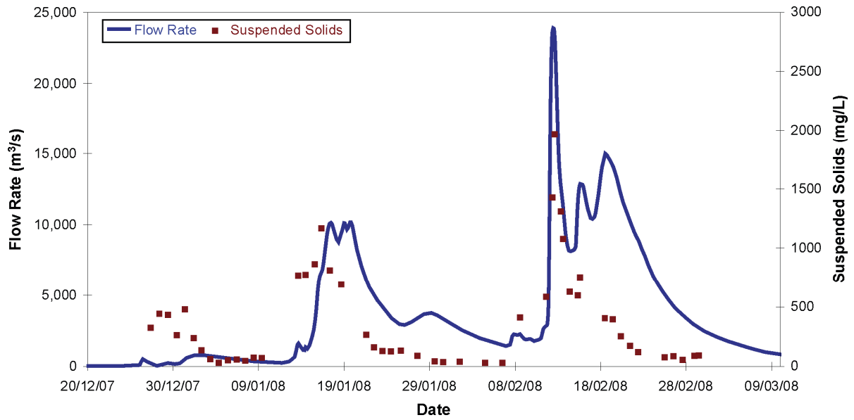
Figure 2: Flow hydrograph for the Burdekin River at Clare in the 2007/08 water year. Total suspended solid (TSS) samples (concentrations shown in mg/L) were collected from the Inkerman Bridge throughout the flow to calculate the sediment load.
